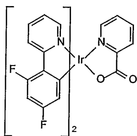
FIr(pic)
