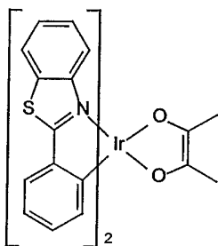
Bt 2 (acac)
