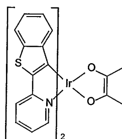
Btp 2 (acac)
