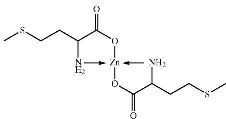
[Chemical Formula 1]
