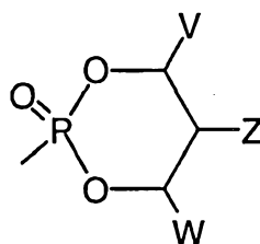
Formula G
