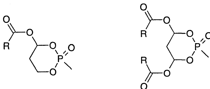
Formula B
