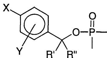
Formula D
