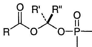
Formula A
