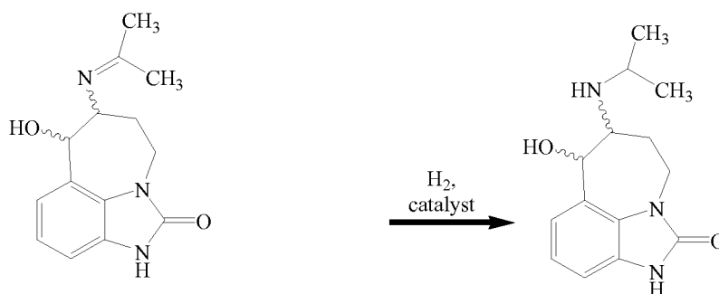
trans -7-[isopropyl imino]-6-hydroxy-6,7,8,9-tetrahydro-2H-2,9a-diazabenz[cd]azulen-1-one
