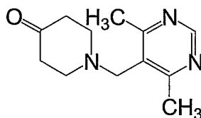
Formula VIIIa
