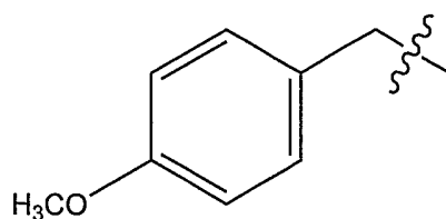
p-Methoxybenzyl (PMB)
