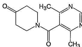
Formula VIIIa
