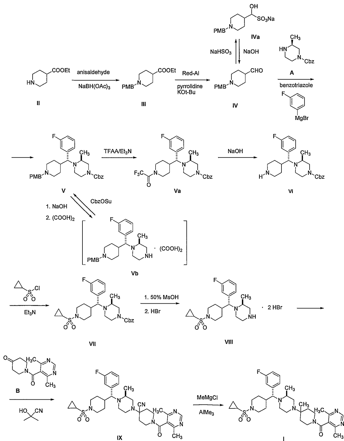
Scheme I
