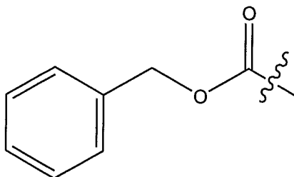
Carbobenzyloxy (Cbz)
