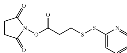
N-succinimidyl-3-(2-pyridyldithio)propionate (SPDP),
