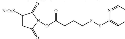
N-succinimidyl-4-(2-pyridyldithio)2-sulfo-butanoate (sulfo-SPDB).
