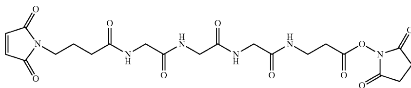
2,5-dioxopyrrolidin-1-yl 17-(2,5-dioxo-2,5-dihydro-1H-pyrrol-1-yl)-5,8,11,14-tetraoxo-4,7,10,13-tetrazaheptadecan-1-oate (CX1-1)
