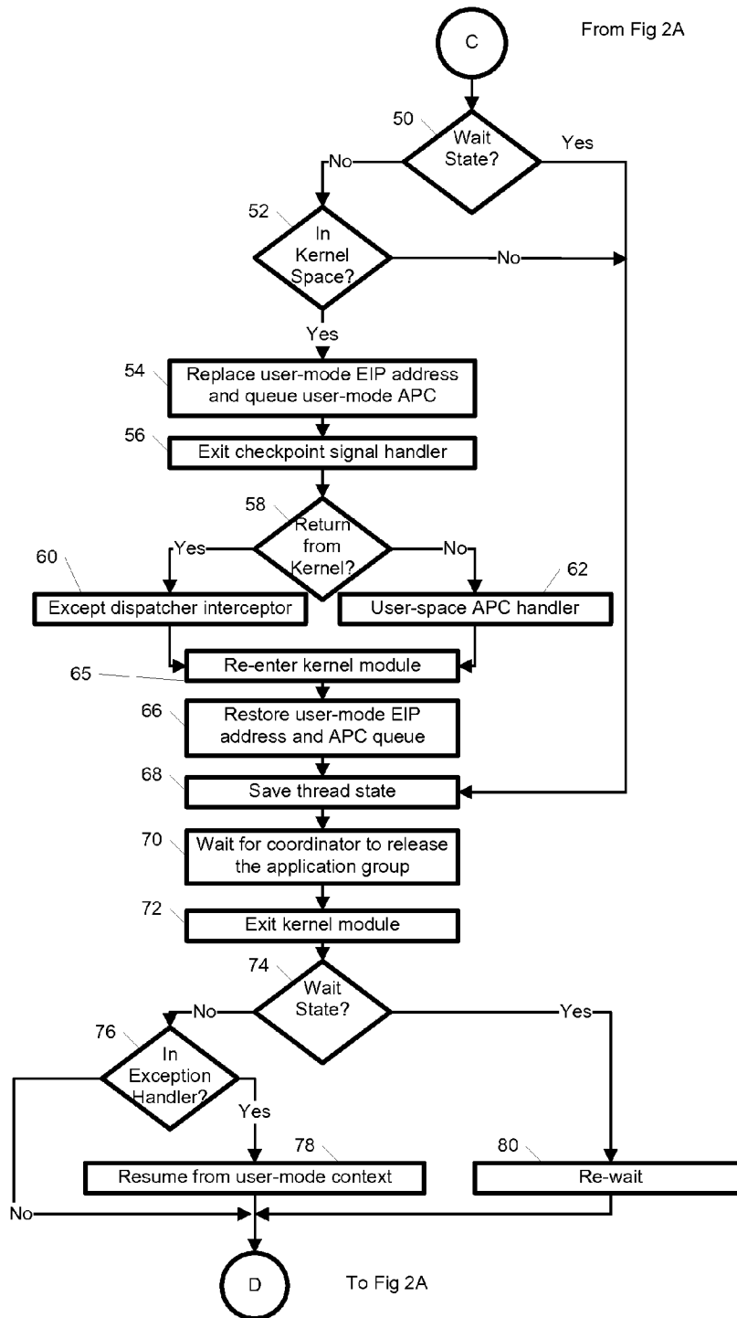
Fig. 2B – Taking an application process' checkpoint
