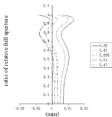
longitudinal aberration curve
