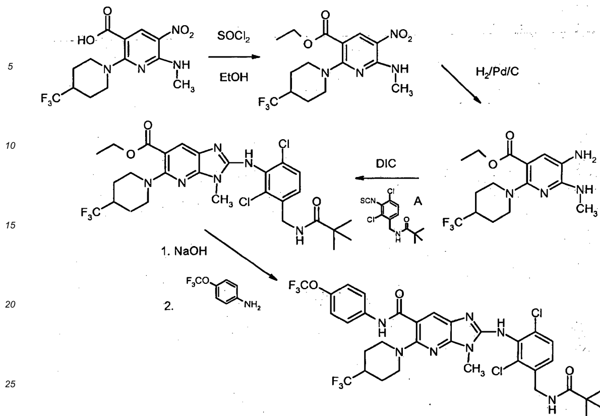
(a) 6-Methylamino-5-nitro-2-(4-trifluoromethyl-piperidinyl)nicotinic acid ethylester
