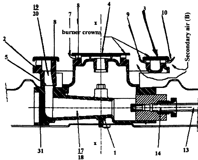
Section B-B
