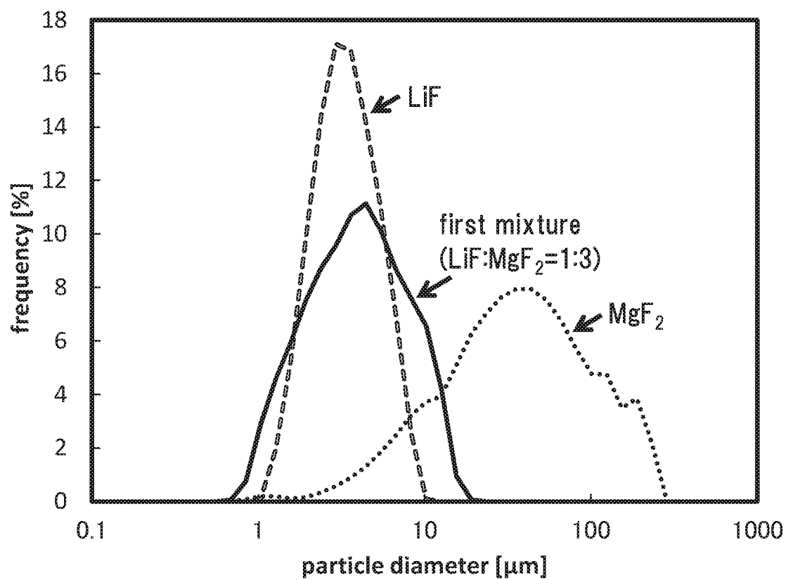
FIG. 29 particle size distribution
