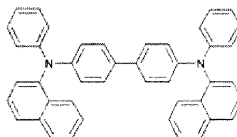
4,4'-bis[N-(1-naphthyl)-N- phenyl-amino]biphenyl (NPD)
