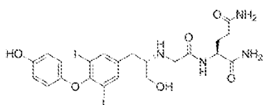
T2AA-Gln
