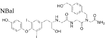
T2AA-Gly-NPip
