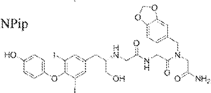
T2AA-NPip-NLys
