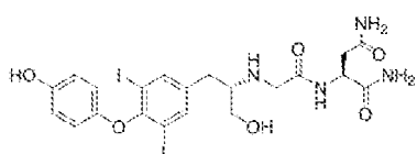
T2AA-Asn
