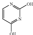
2,4-dihydroxy-pyrimidine
