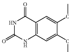
6,7-dimethoxy-quinazolidine-2,4-dione
