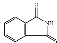
phthalimide
