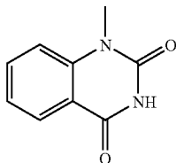
1-N-methyl-quinazolidine-2,4-dione
