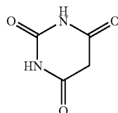
barbituric acid
