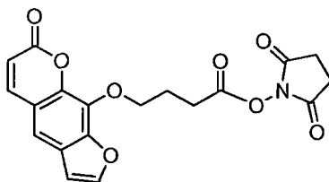
Psoralen linker
