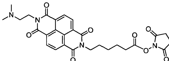
NDI linker
