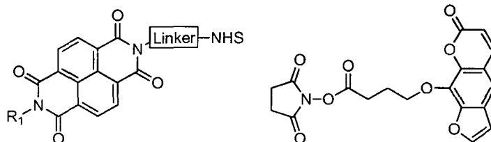
naphthalene diimide NHS ester
