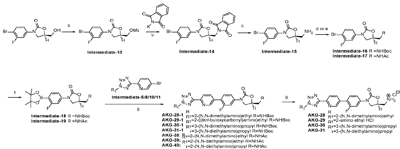
Scheme 5
