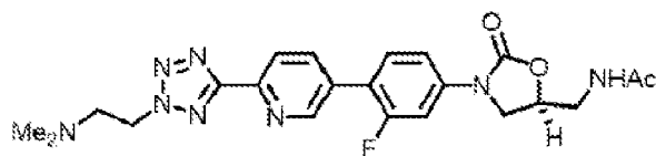
Formula 1c
