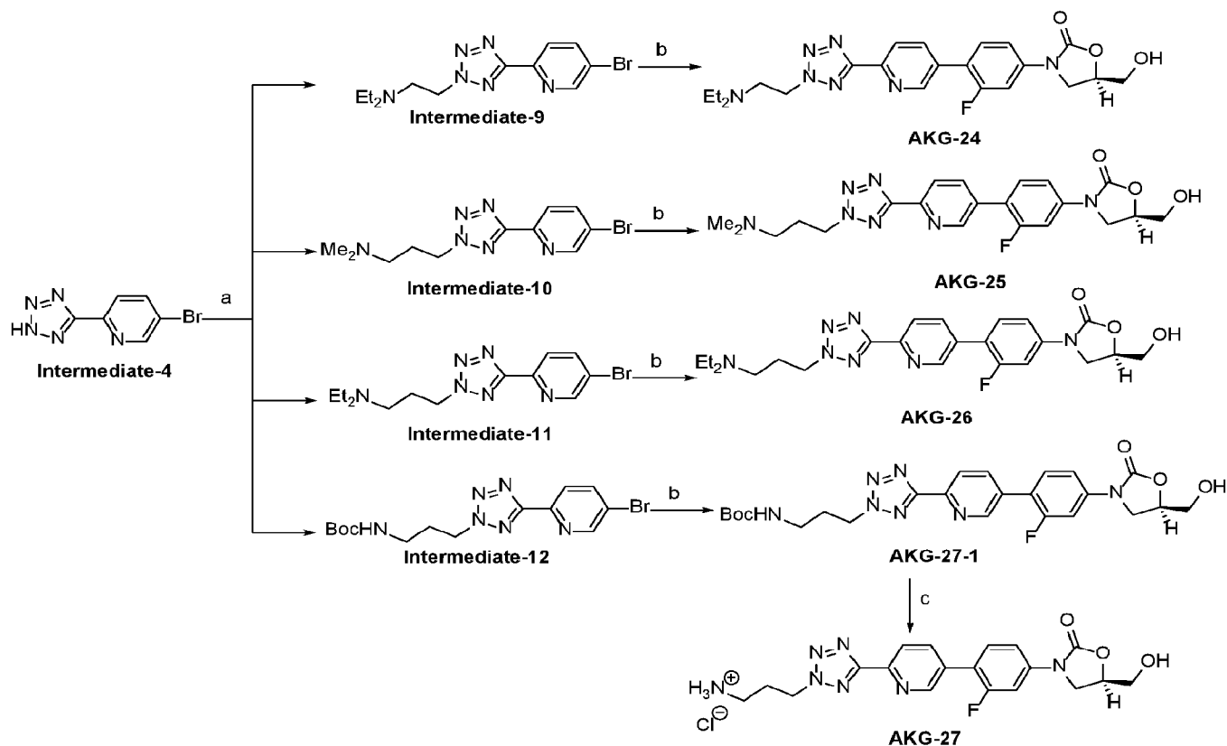
Scheme 5
