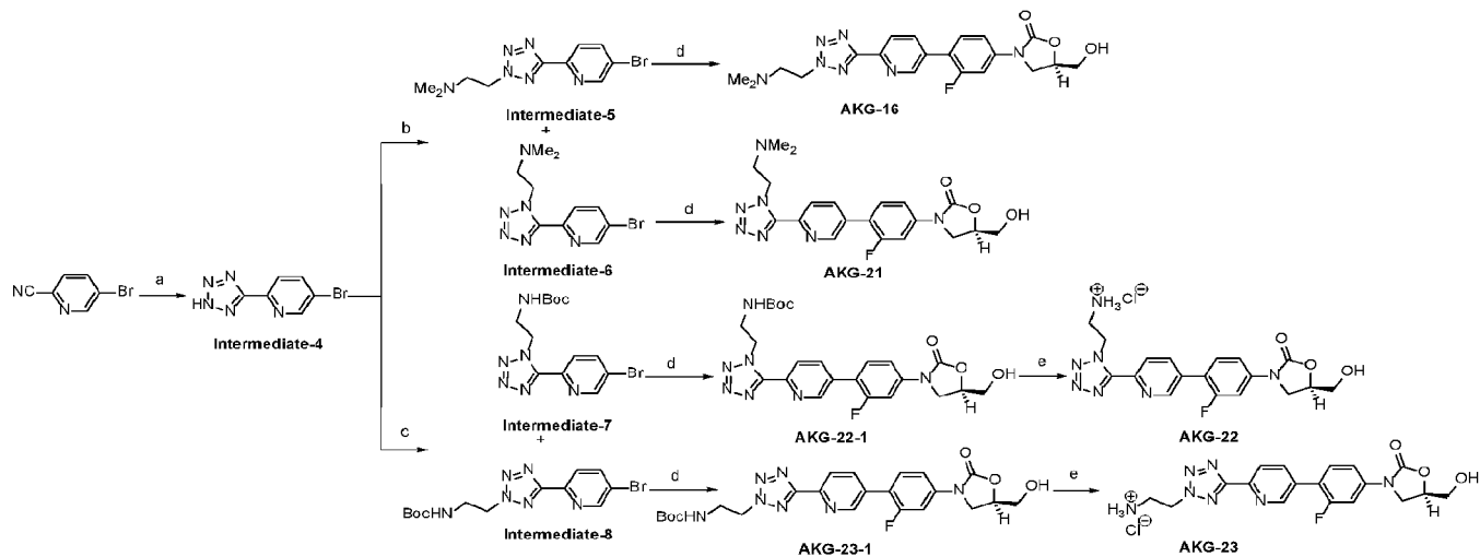
Scheme 3
