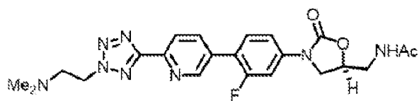
Formula 1c
