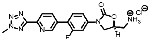
Formula 1a.
