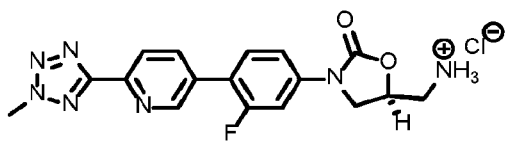
Formula 1a
