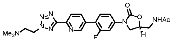
Formula 1c.
