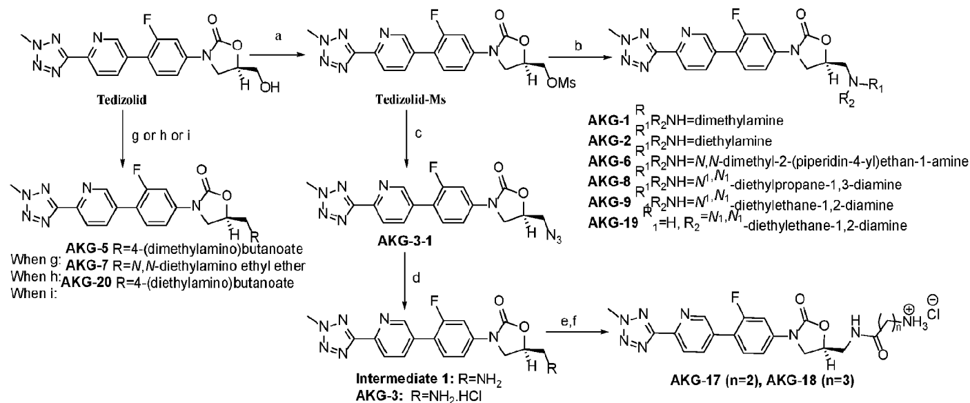
Scheme 1
