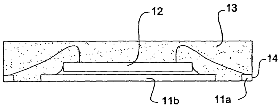
FIG. 3 (PRIOR ART)
