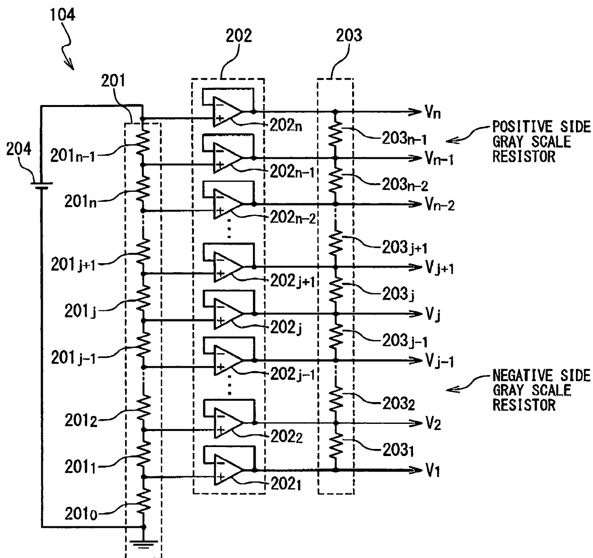
Fig. 2 PRIOR ART
