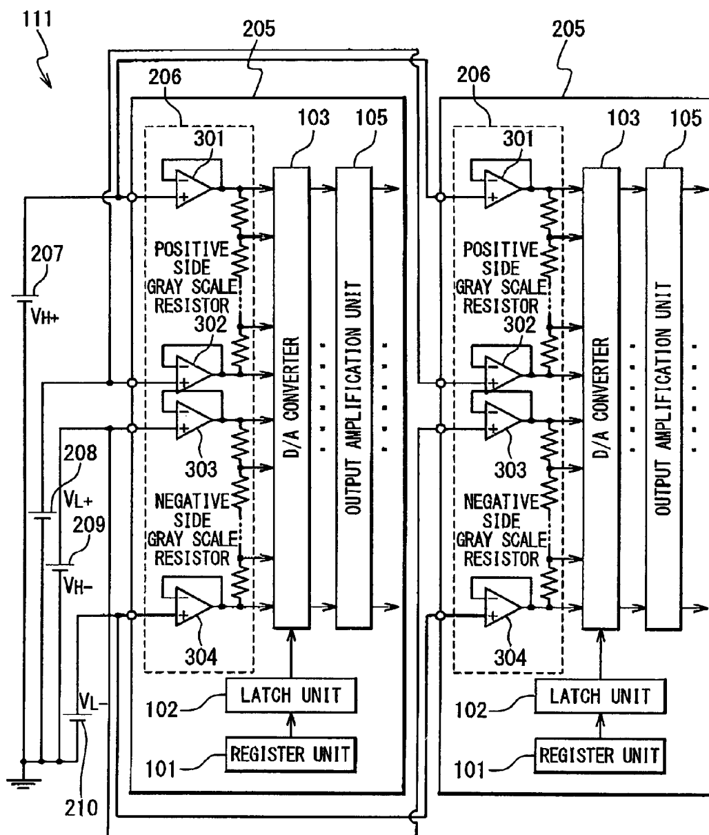
Fig. 3 PRIOR ART
