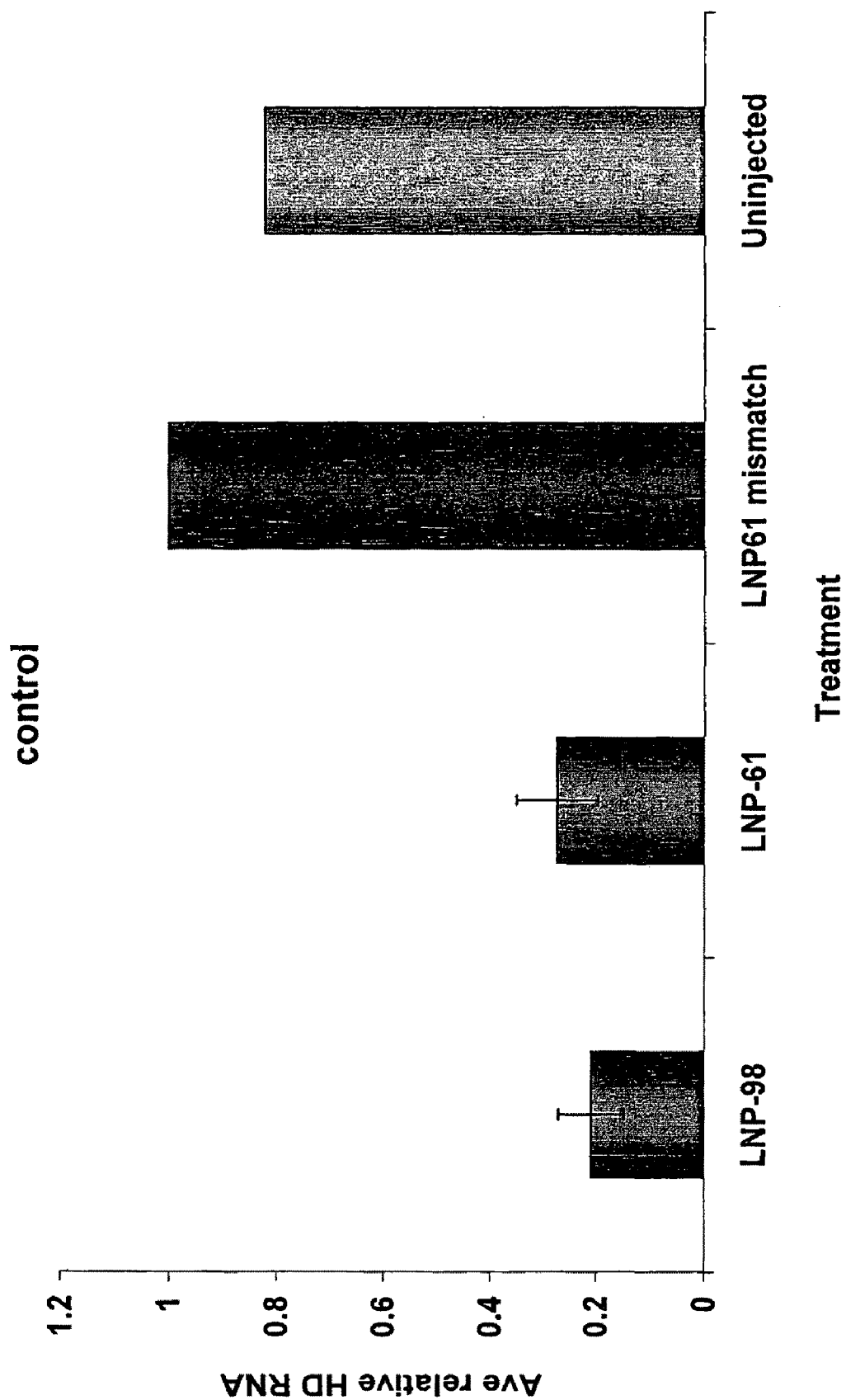
Figure 44: Relative expression of HD RNA with active LNP-98 and LNP-61 formulated active siNA compared to LNP-61 mismatch control
