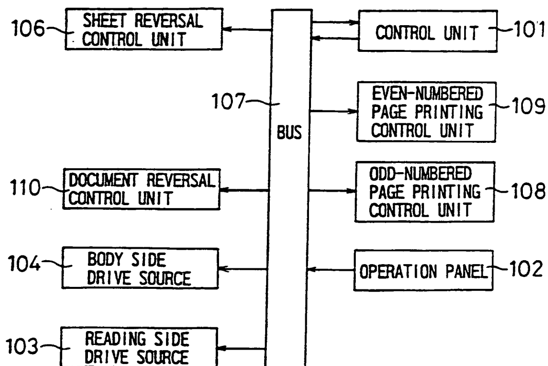
FIG. 17 PRIOR ART
