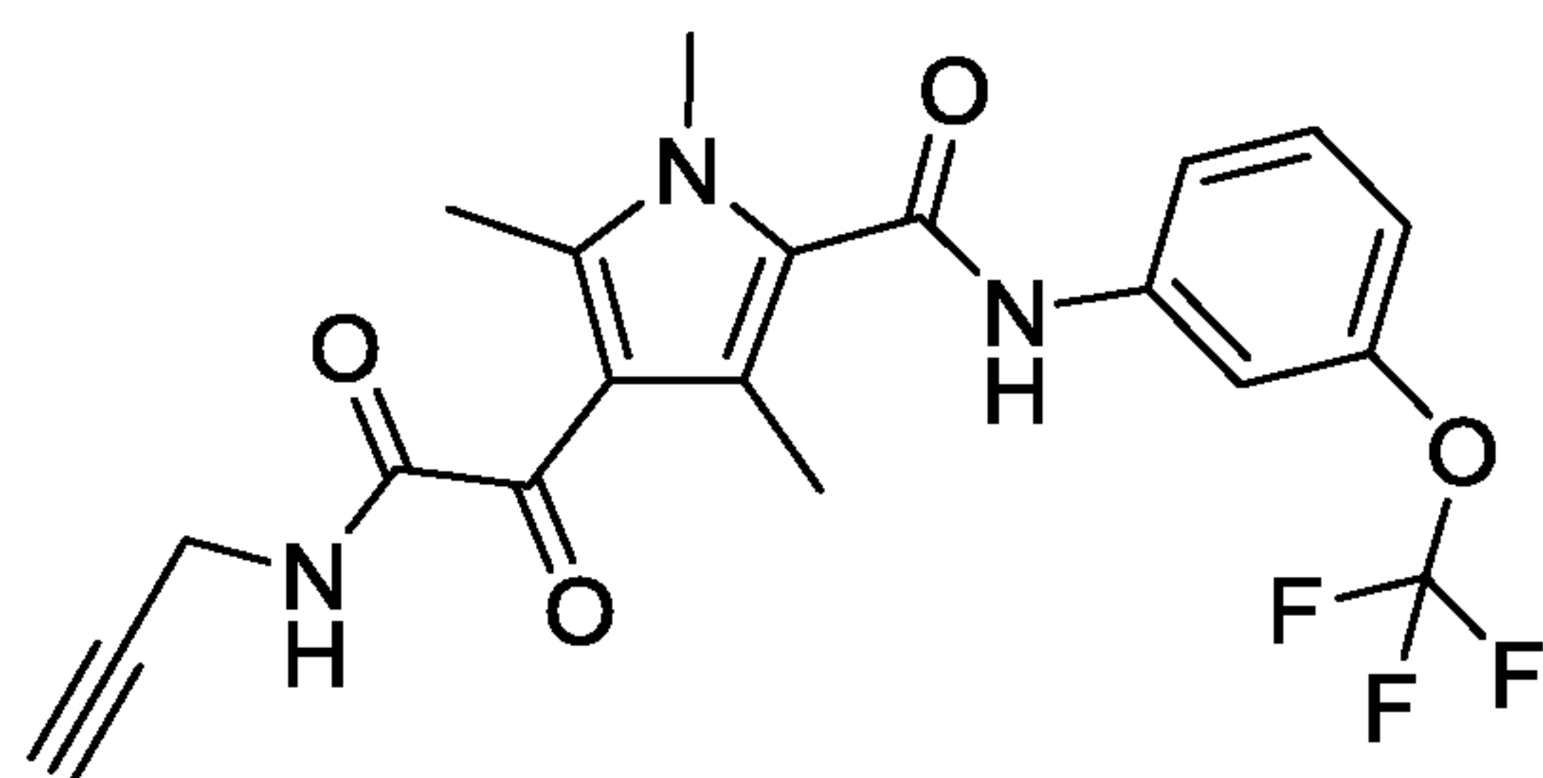
1,3,5-trimethyl-4-(2-oxo-2-(prop-2-yn-1-ylamino)acetyl)-N-(3-(trifluoromethoxy)phenyl)-1H-pyrrole-2-carboxamide ( 55 )
