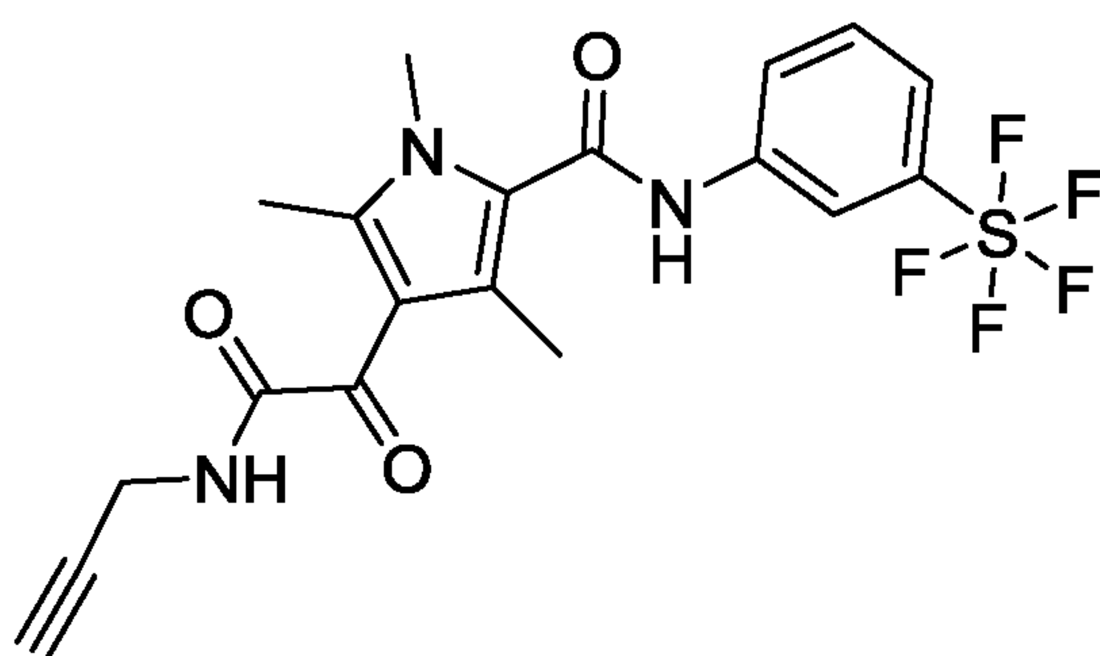
1,3,5-trimethyl-4-(2-oxo-2-(prop-2-yn-1-ylamino)acetyl)-N-(3-(pentafluorosulfanyl)phenyl)-1H-pyrrole-2-carboxamide (60)
