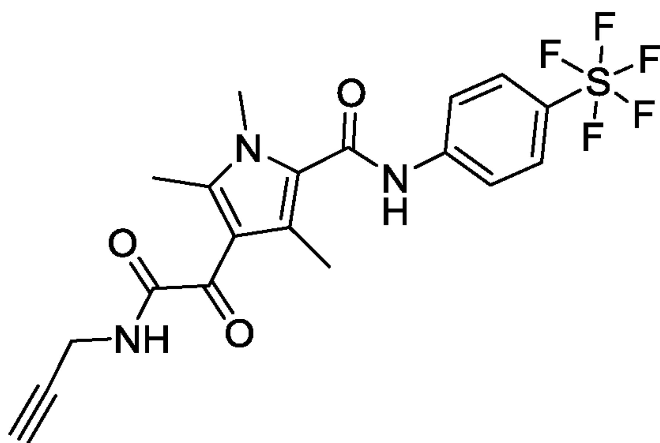
1,3,5-trimethyl-4-(2-oxo-2-(prop-2-yn-1-ylamino)acetyl)-N-(4-(pentafluorosulfanyl)phenyl)-1H-pyrrole-2-carboxamide (59)
