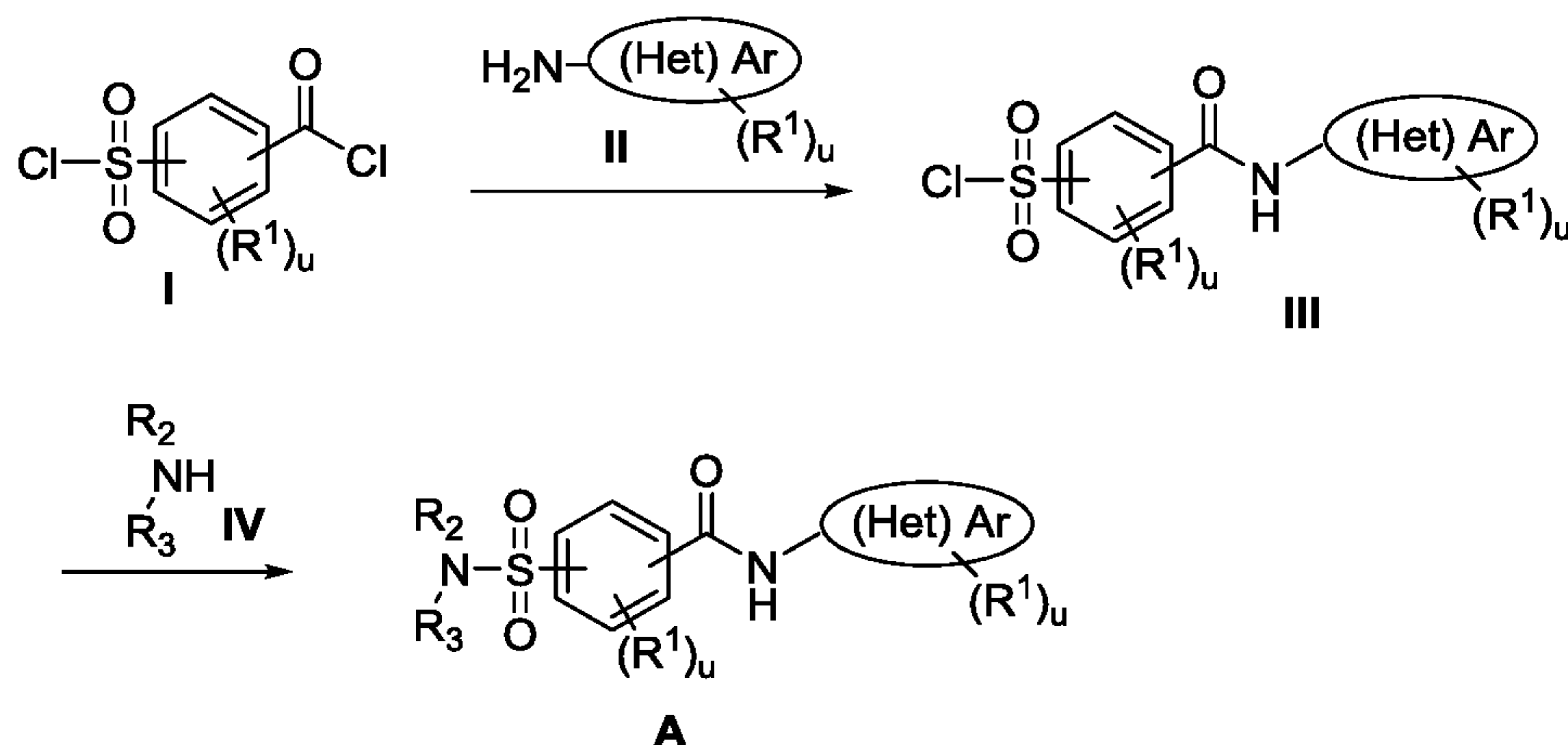
Scheme 1 A synthetic approach to compound A
