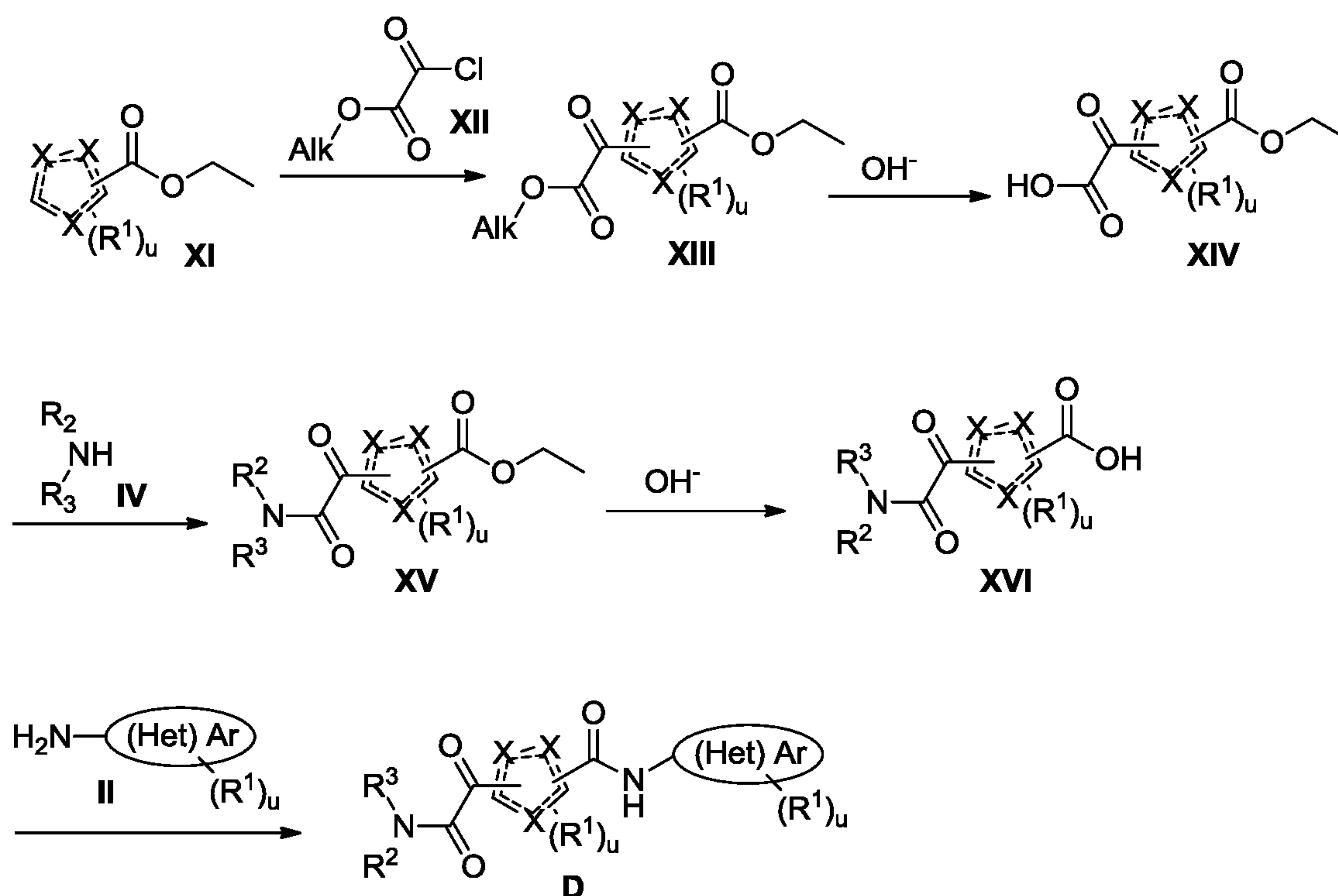
Scheme 4 A synthetic approach to compound D
