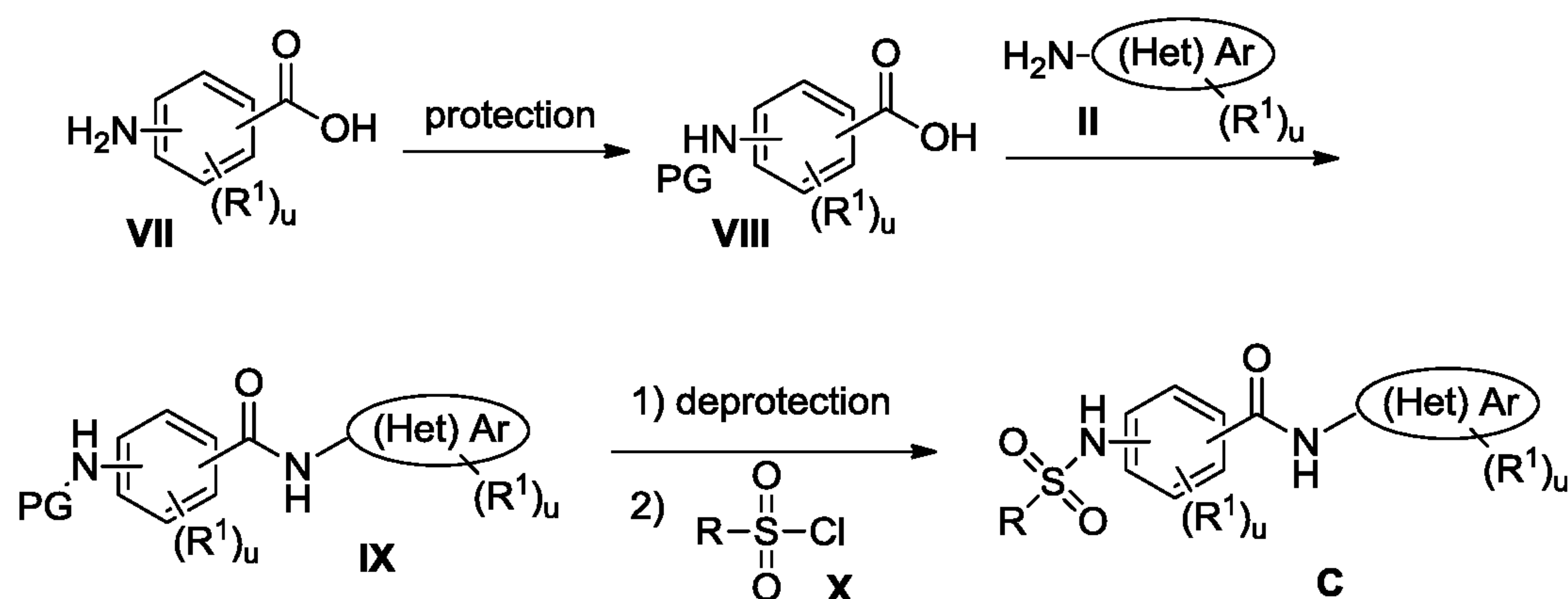
Scheme 3 A synthetic approach to compound C
