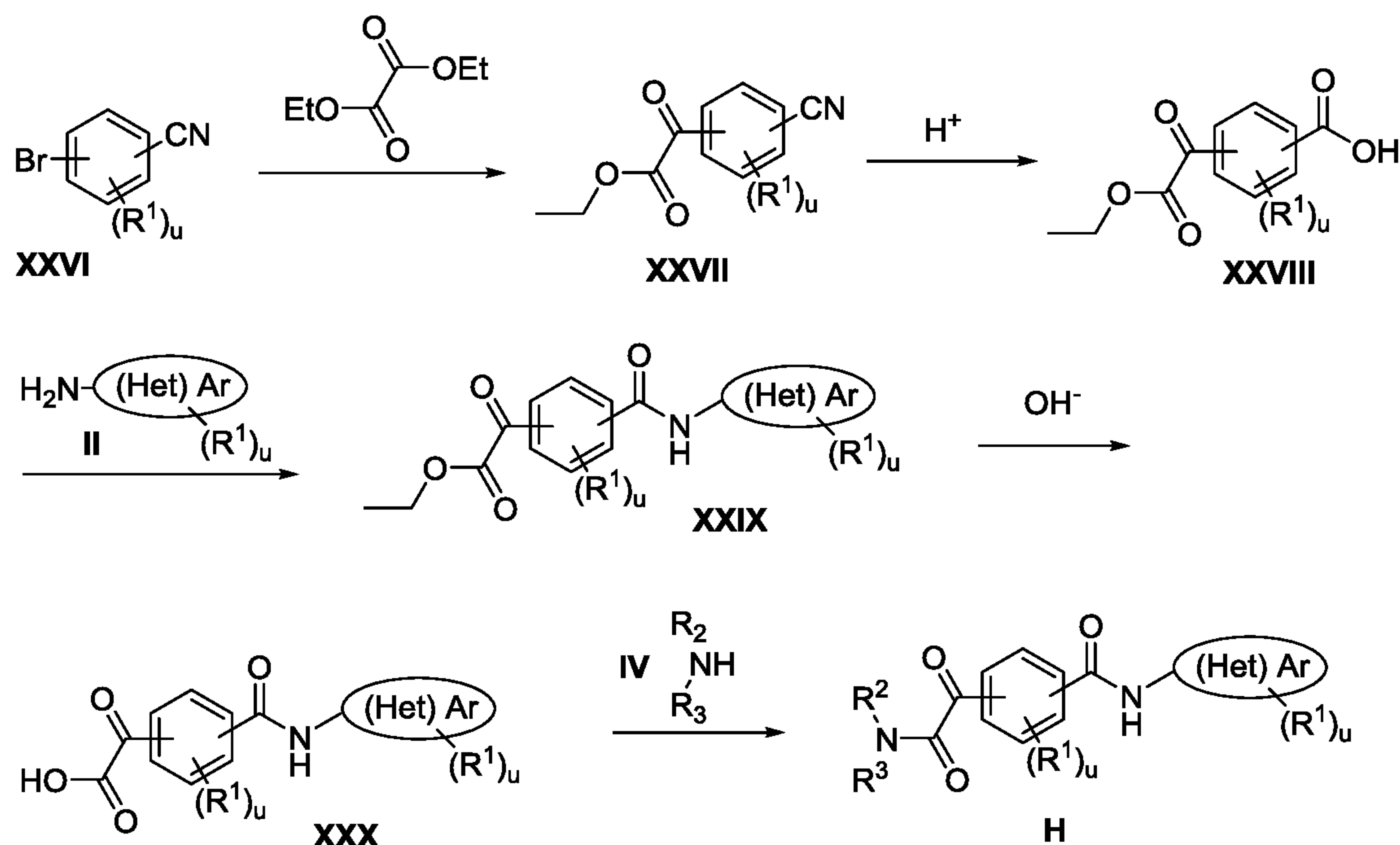
Scheme 7 A synthetic approach to compounds H
