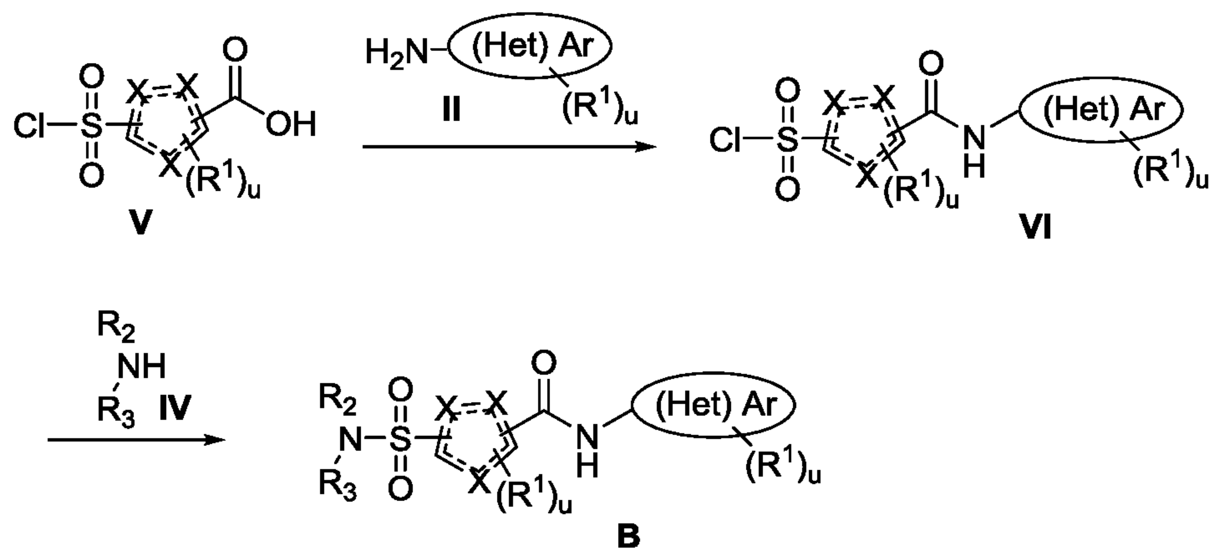
Scheme 2 A synthetic approach to compound B
