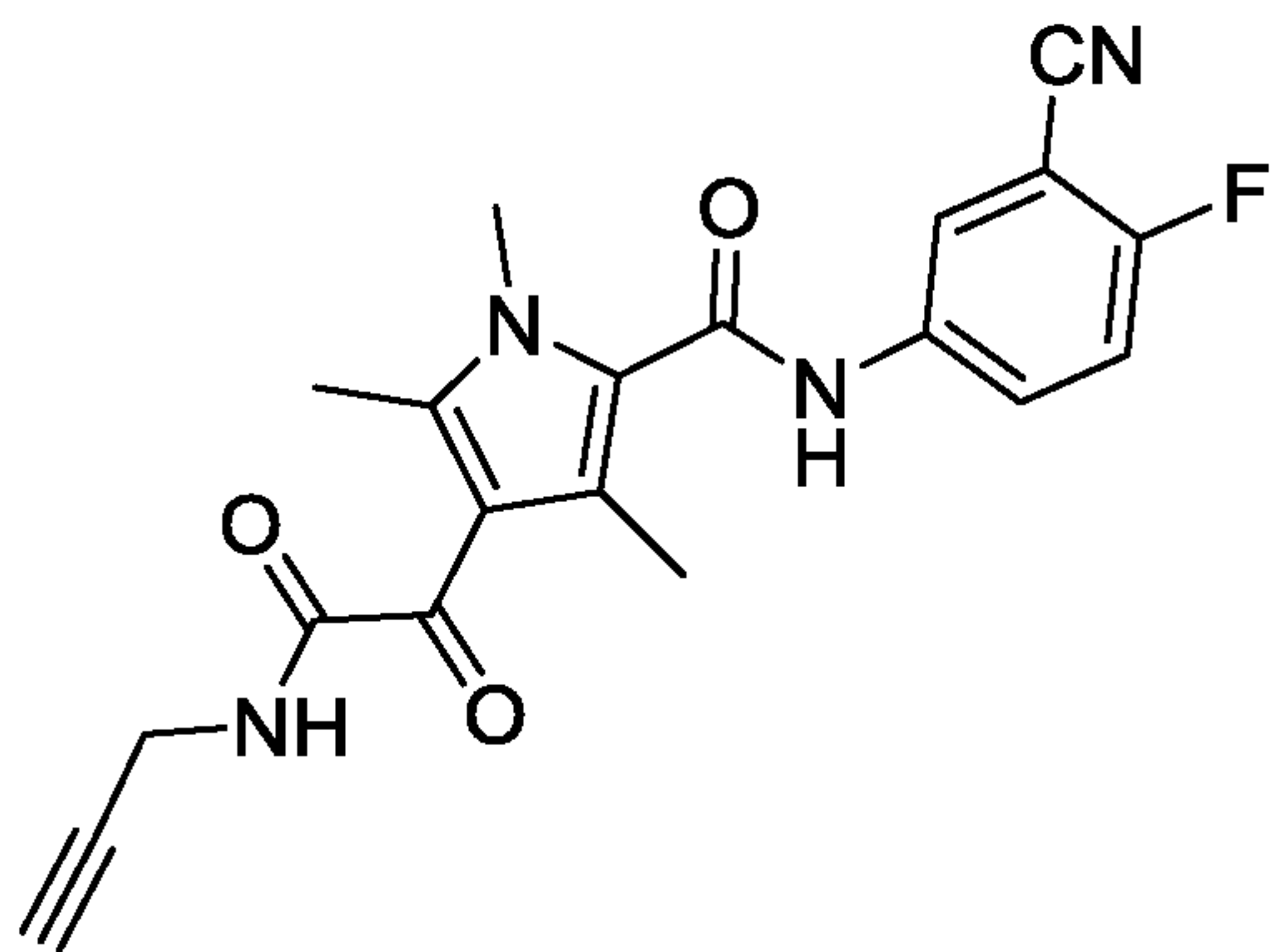
N -(3-cyano-4-fluorophenyl)-1,3,5-trimethyl-4-(2-oxo-2-(prop-2-yn-1-ylamino)acetyl)-1 H -pyrrole-2-carboxamide ( 65 )
