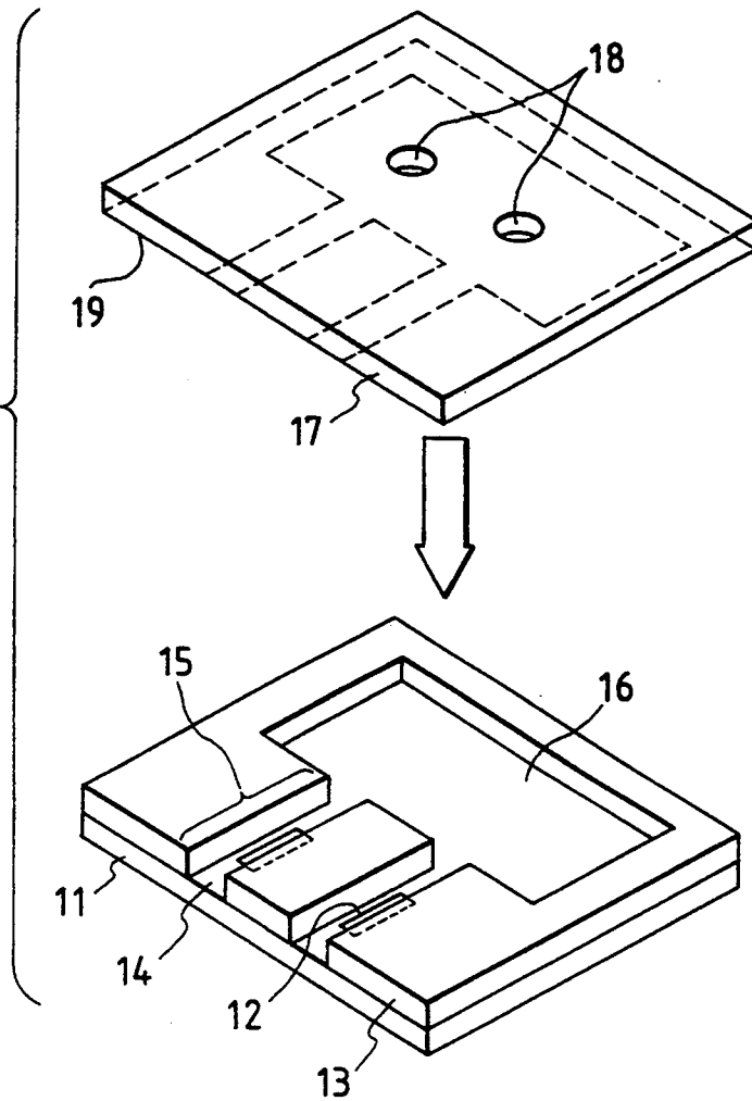
FIG. 1 PRIOR ART
