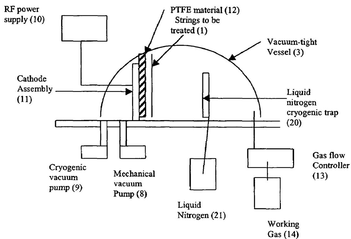
FIG 1: PLASMA SPUTTER DEPOSITION SYSTEM
