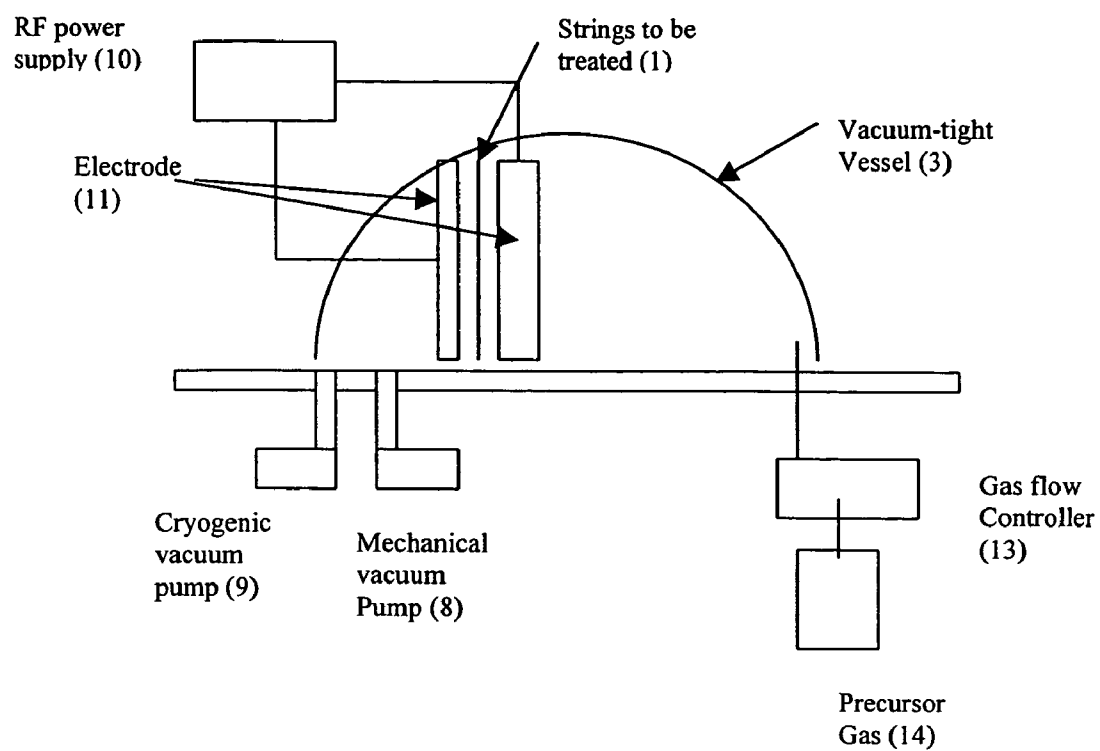
FIG 4: PLASMA CHEMICAL VAPOR DEPOSITION SYSTEM
