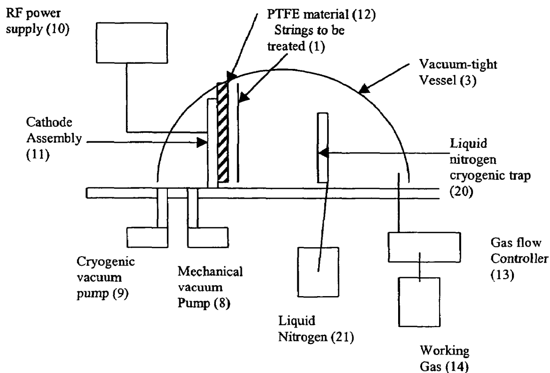
PLASMA SPUTTER DEPOSITION SYSTEM
