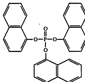
Trinaphthyl Phosphate
