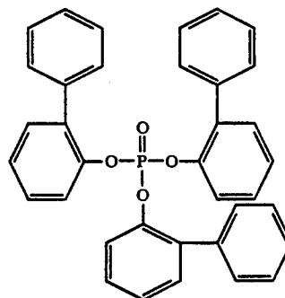
Tris Ortho-biphenyl Phosphate
