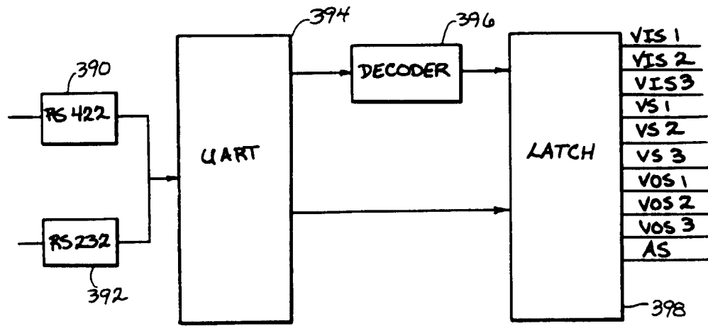
CONTROL DECODER
