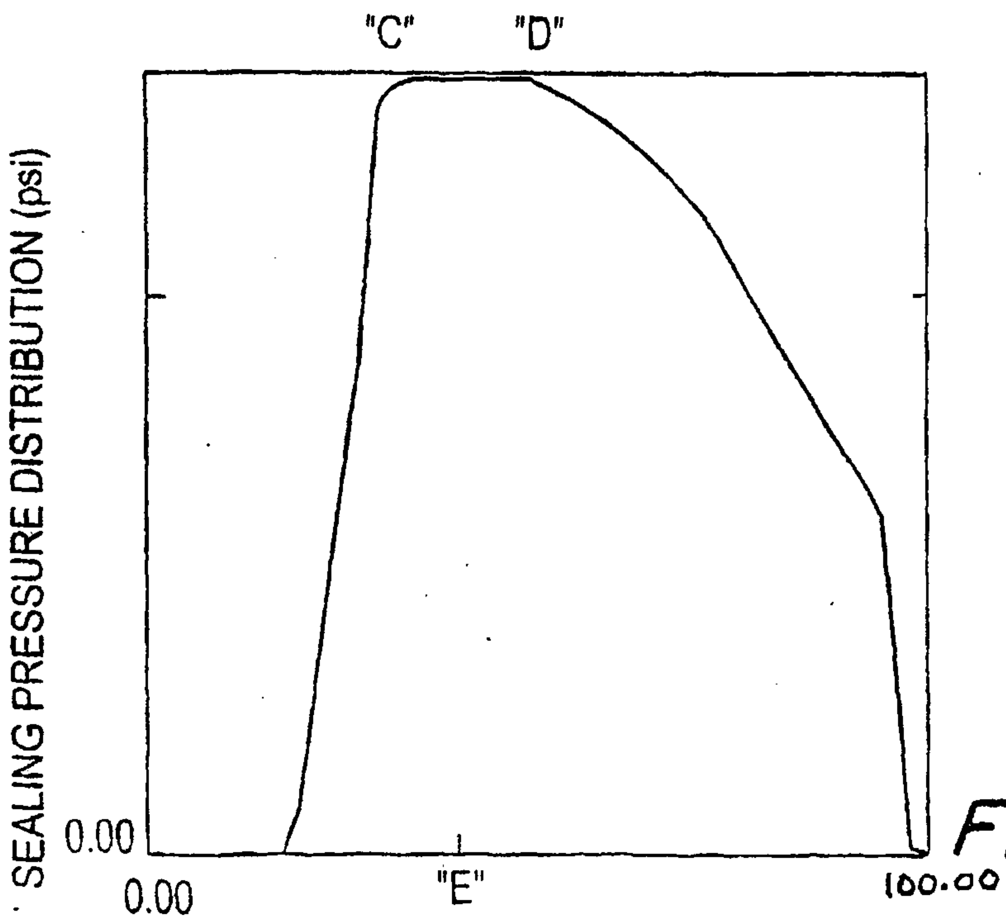
% DISTANCE FROM END OF LIP TO END OF FLANGE FLANGE SEALING SURFACE WITHOUT LUBRICANT GROOVE
