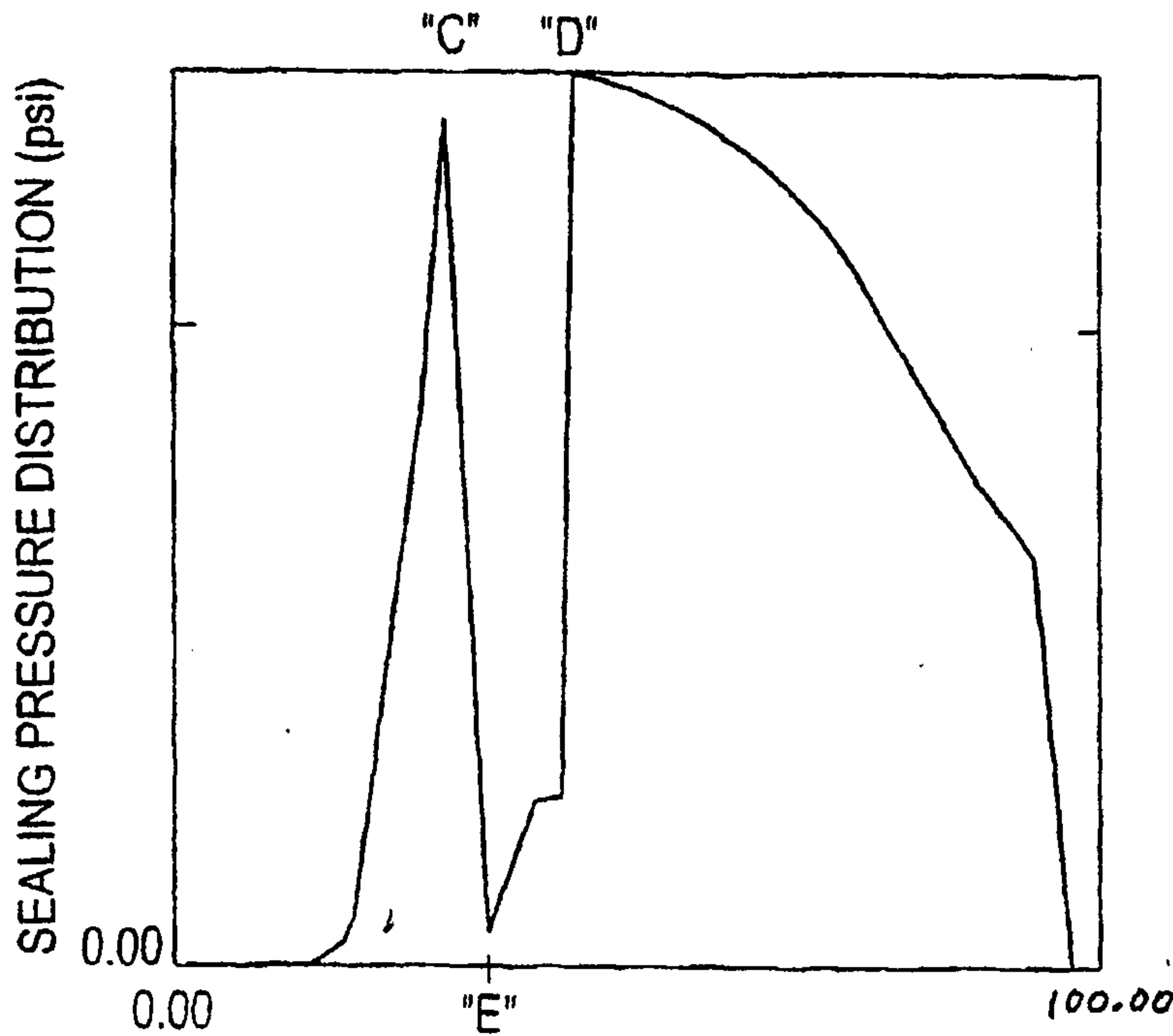
% DISTANCE FROM END OF LIP TO END OF FLANGE FLANGE SEALING SURFACE WITH LUBRICANT GROOVE
