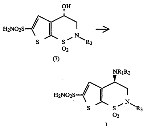
Step 7 C(6)-Sulfonamide protection/C(4)-hydroxyl activation/displacement
