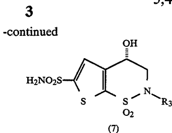
Step 7 C(6)-Sulfonamide protection/C(4)-hydroxyl activation/displacement
