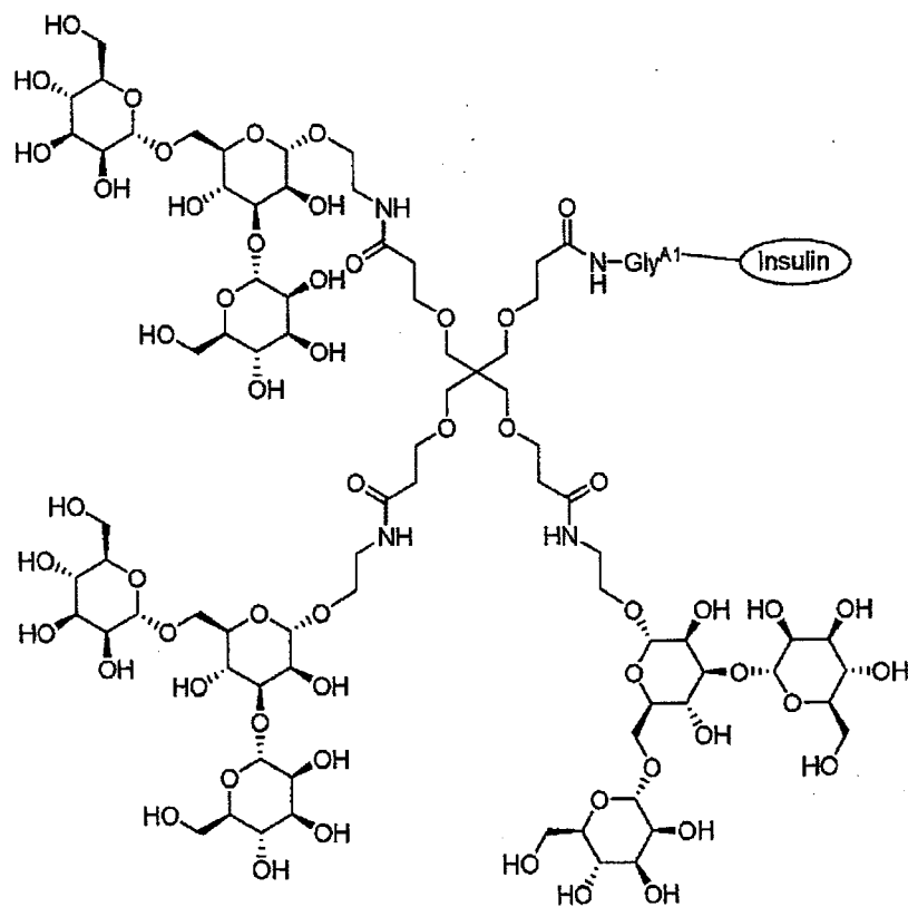
Conjugate I-14 TSPE-AETM-3 (A1)
