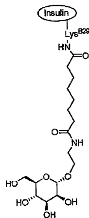
Conjugate I-8 DSS-AEM-1 (B29) Figure 45 (continued)
