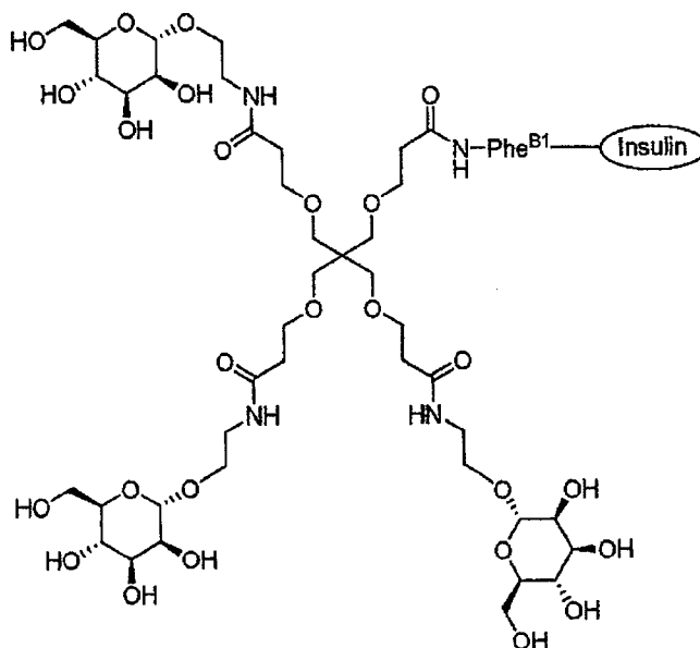
Conjugate I-16 TSPE-AEM-3 (B1)
