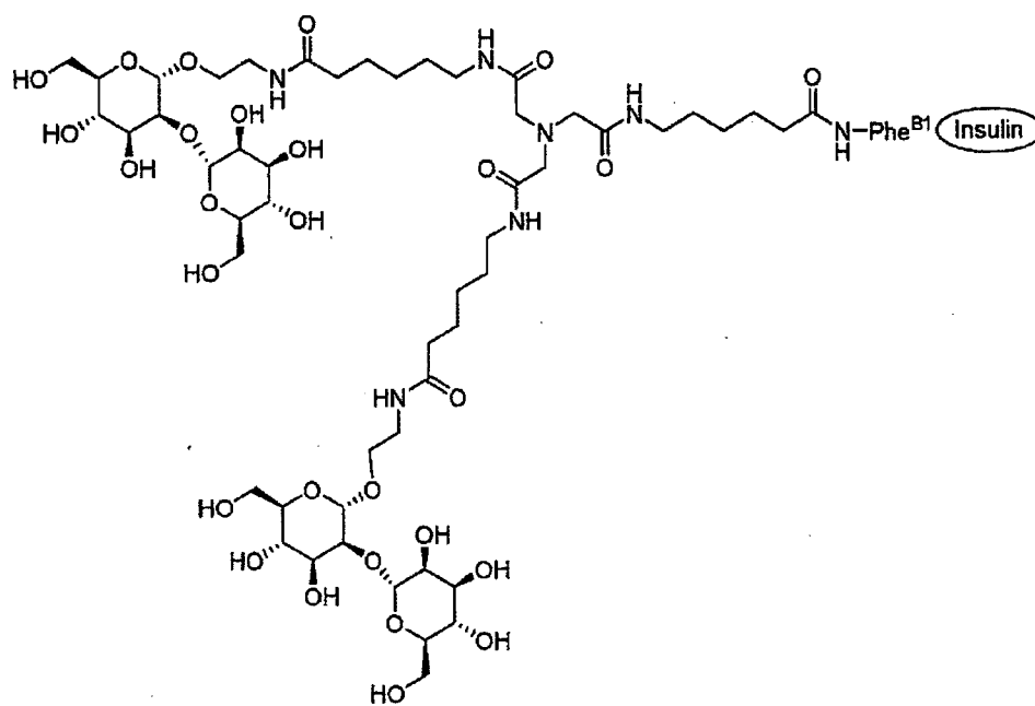
Conjugate I-3 TSAT-C6-AEBM-2 (B1)
