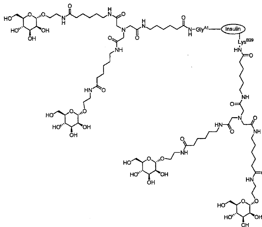
Conjugate II-1 TSAT-C6-Di-sub-AEM-2 (A1,B29)
