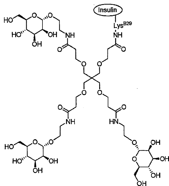
Conjugate I-9 TSPE-AEM-3 (B29)
