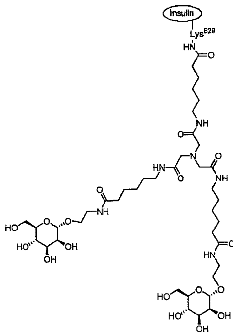
Conjugate I-7 TSAT-C6-AEM-2 (B29)
