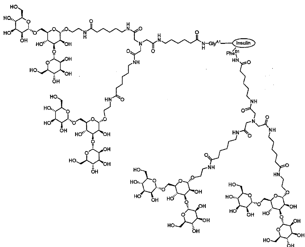
Conjugate II-5 TSAT-C6-Di-sub-AETM-2 (A1,B1)
