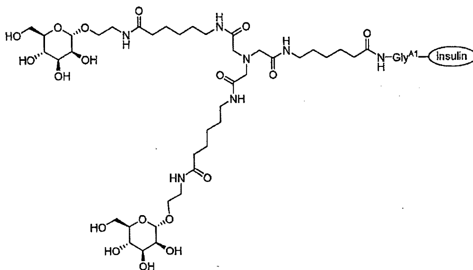
Conjugate I-13 TSAT-C6-AEM-2 (A1)
