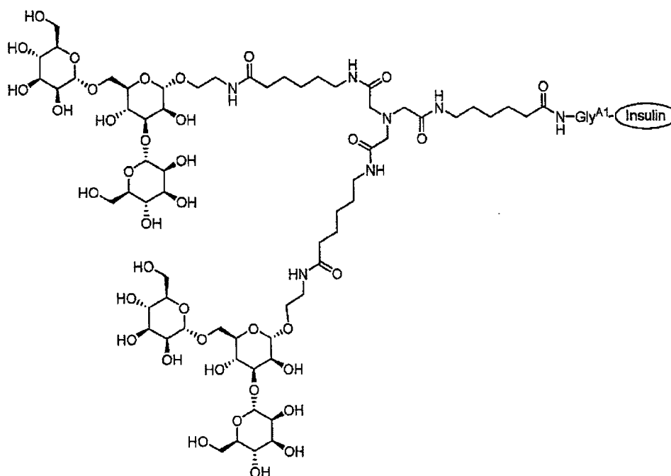
Conjugate I-12 TSAT-C6-AETM-2 (A1)
