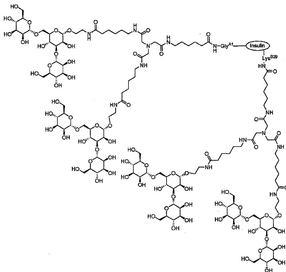
Conjugate II-2 TSAT-C6-Di-sub-AETM-2 (A1,B29)
