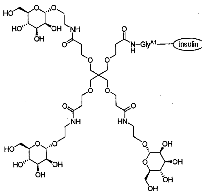
Conjugate I-15 TSPE-AEM-3 (A1)
