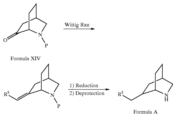
Scheme 8
