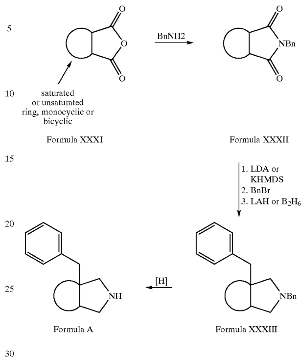
Scheme 15
