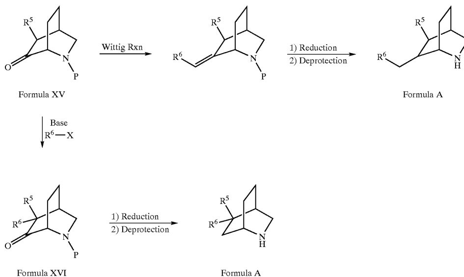
Scheme 10
