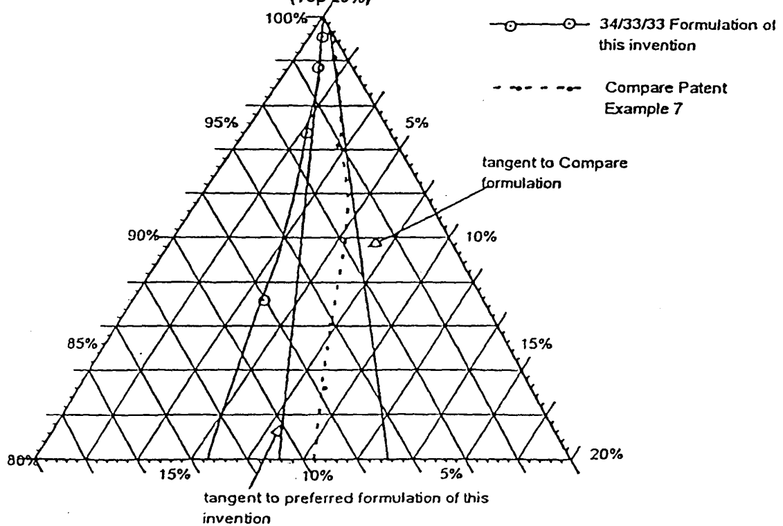
Figure 8 Comparison of Formulation from U.S. 5,746,783 to Preferred Formulation of This Invention (Top 20%)
