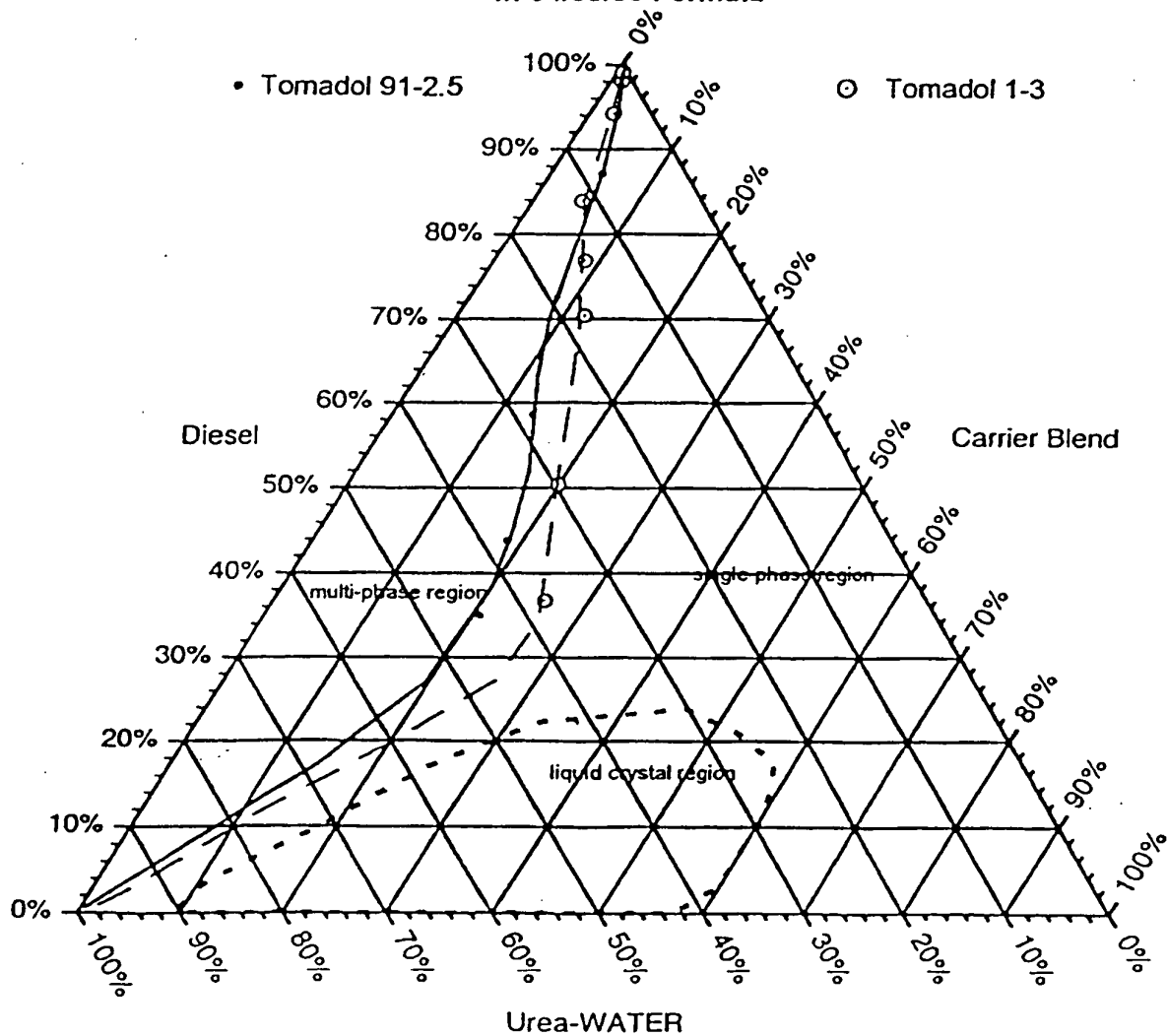
Figure 4 Tomadol 1-3 vs Tomadol 91-2.5 in 34/33/33 Formula
