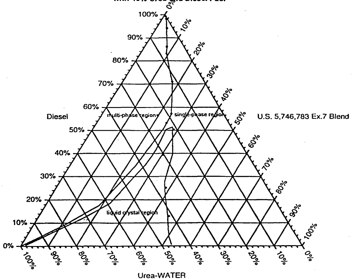
Figure 7 Formulation from U.S. Patent 5,746,783 with 40% Urea and Diesel Fuel
