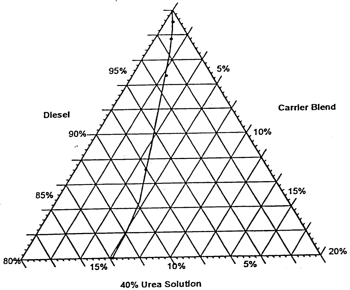
Figure 3. Top 20% of 34/33/33 Ternary Phase Diagram
