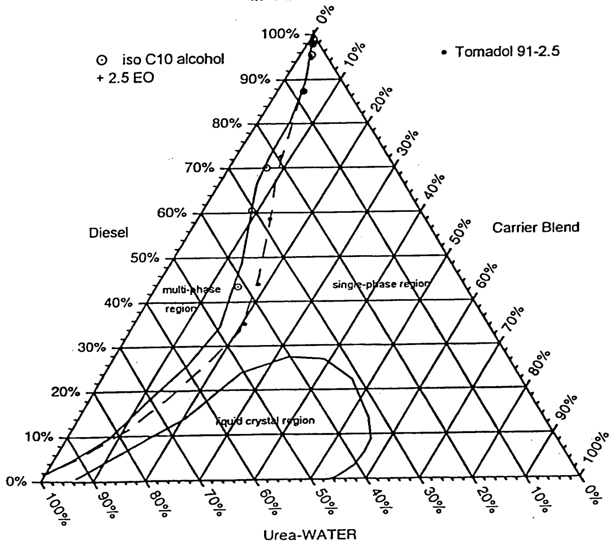
Figure 5 Iso C10 Alcohol + 2.5 EO in 34/33/33 Formula
