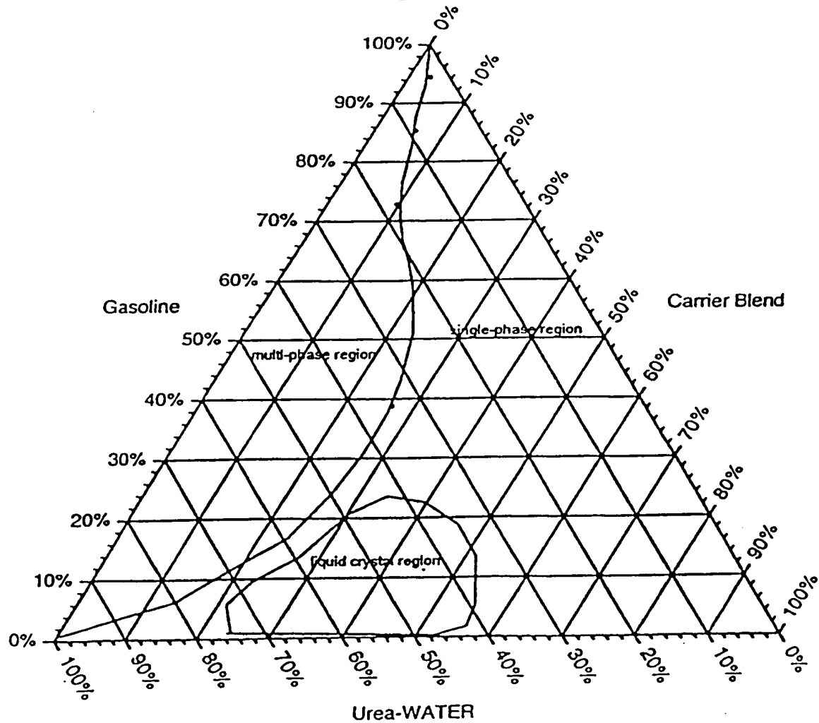
Figure 6 34/33/33 Formula In Gasoline
