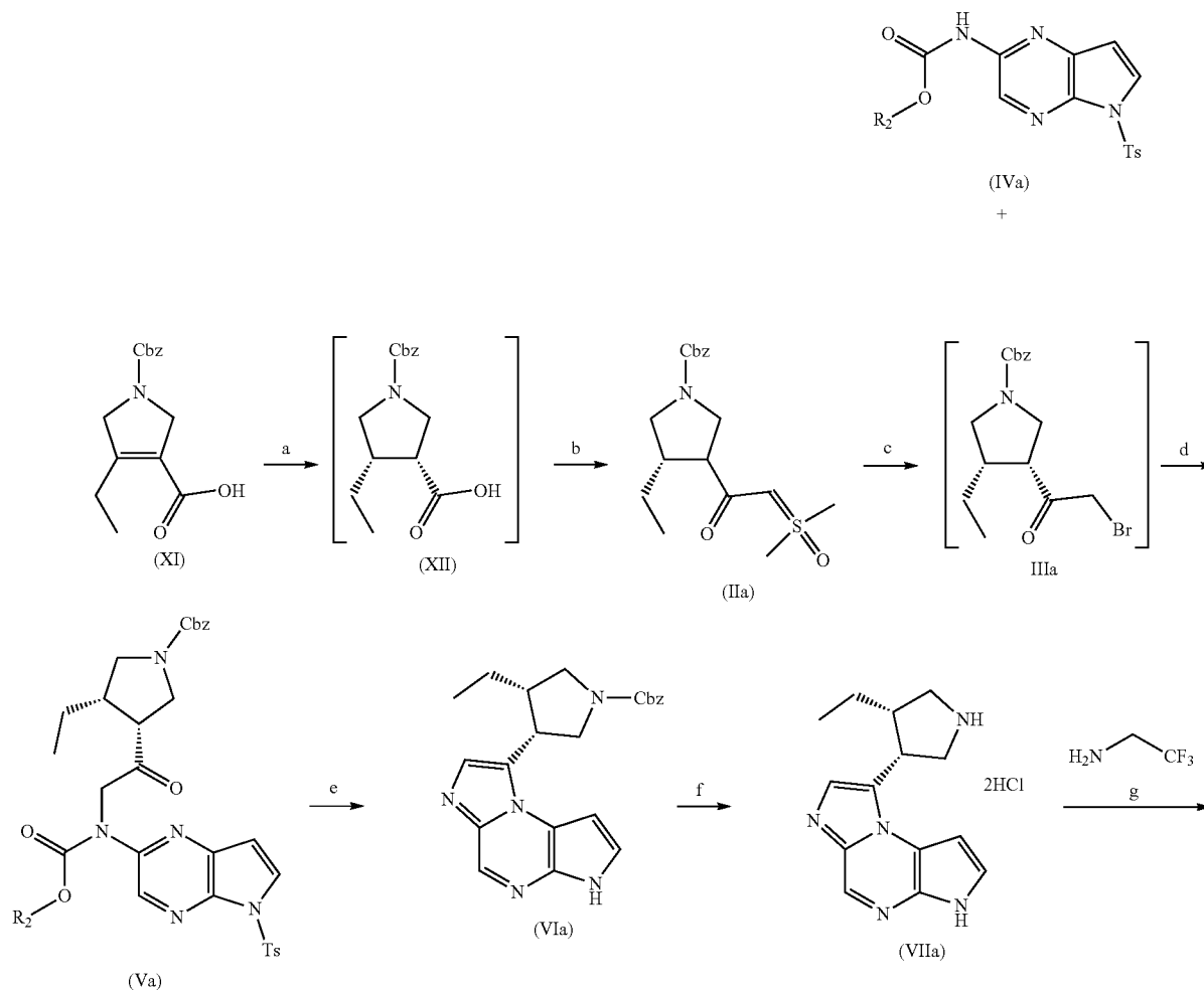
Scheme IIIa
