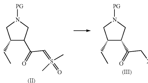
Scheme IX
