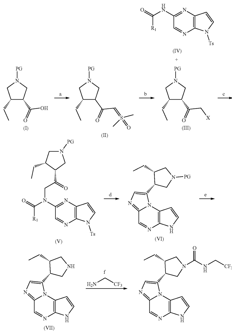
Scheme I
