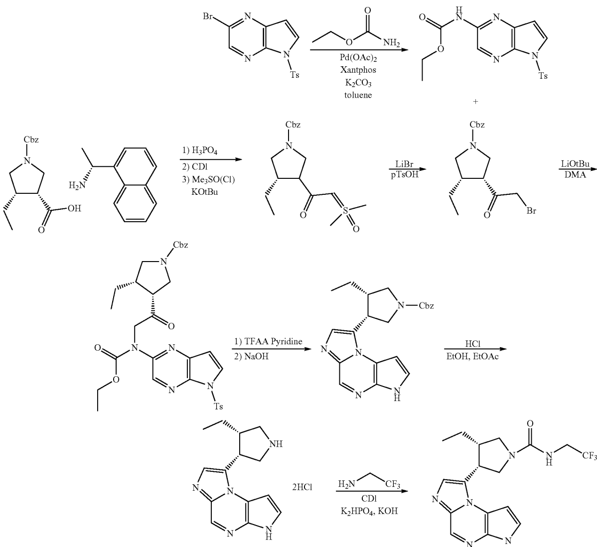
Scheme XV
