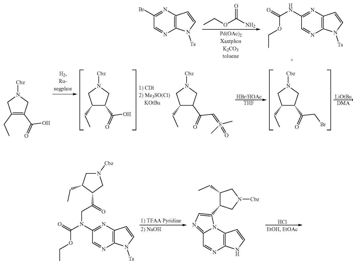
SCHEME XVI
