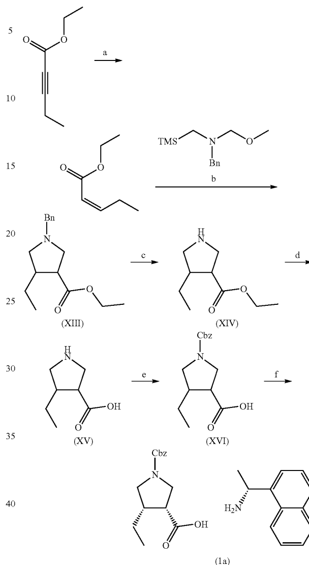
Scheme IV
