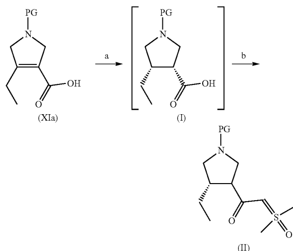
Scheme VIII
