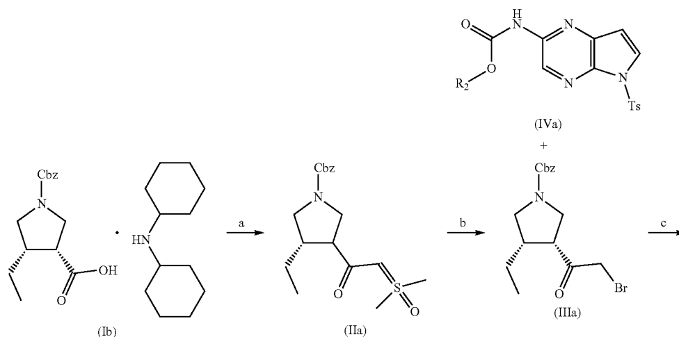
Scheme Ia
