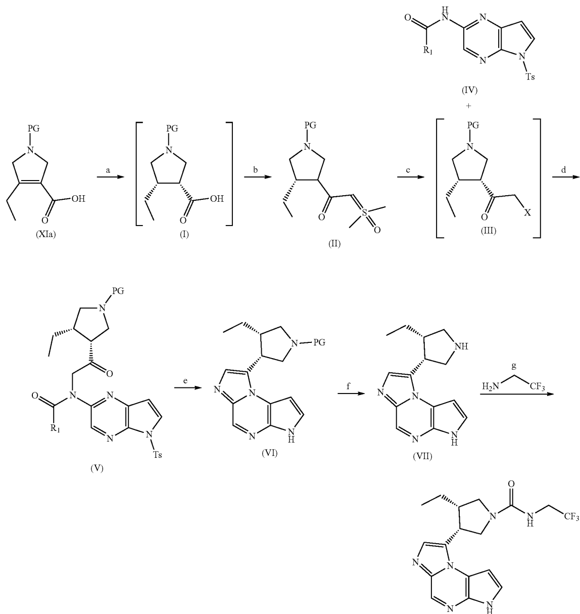
Scheme III
