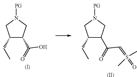
Scheme VII
