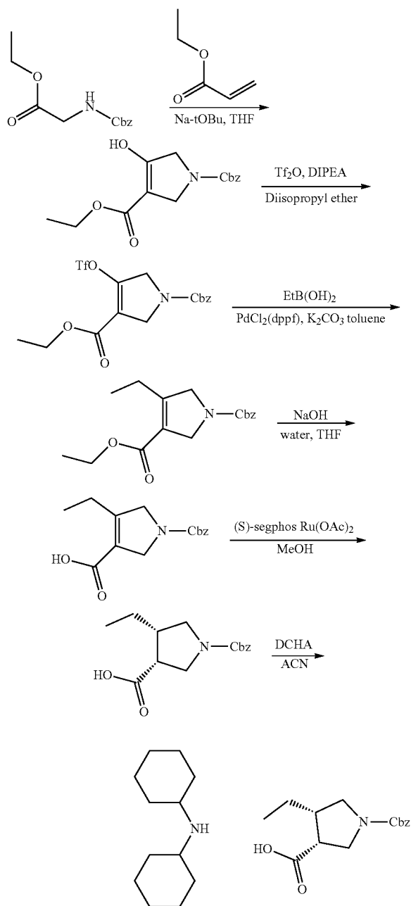
Scheme XIV
