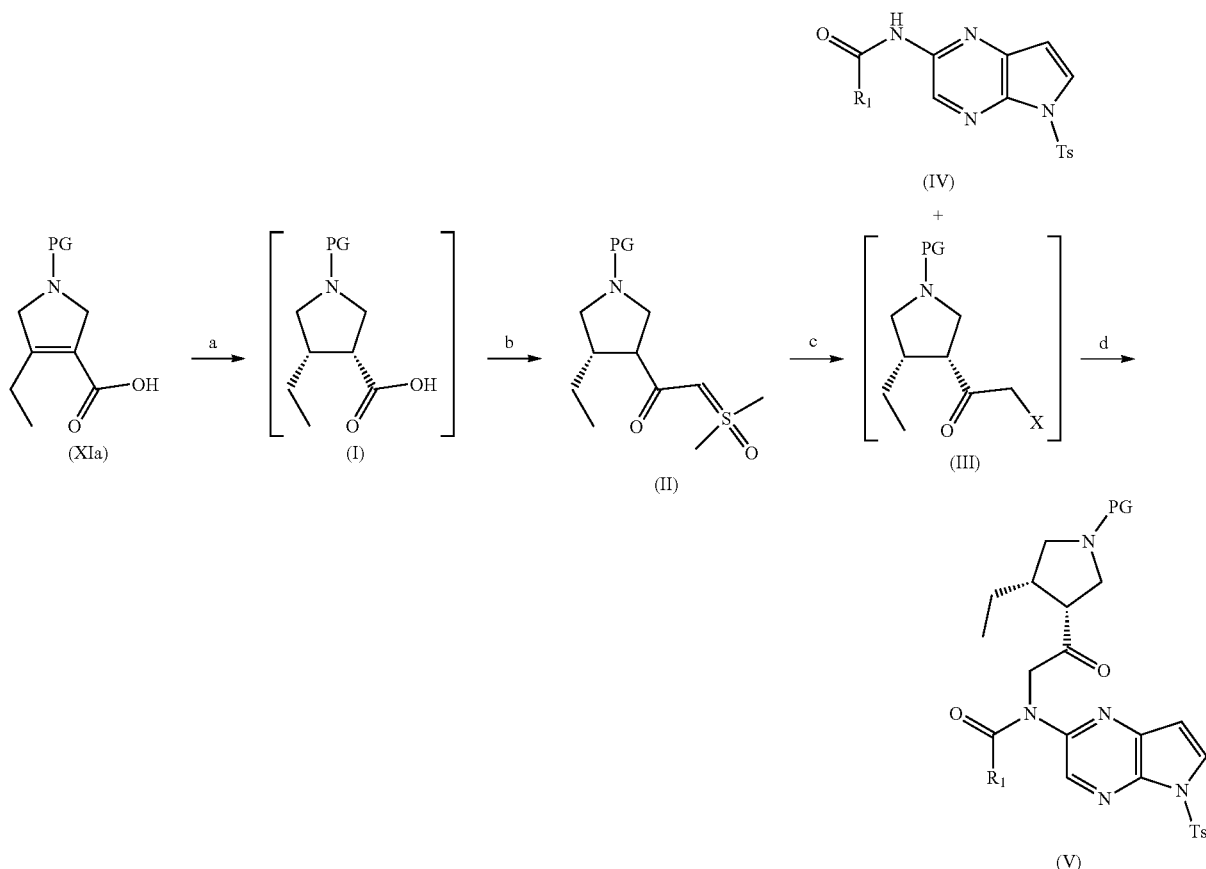
Scheme XIII
