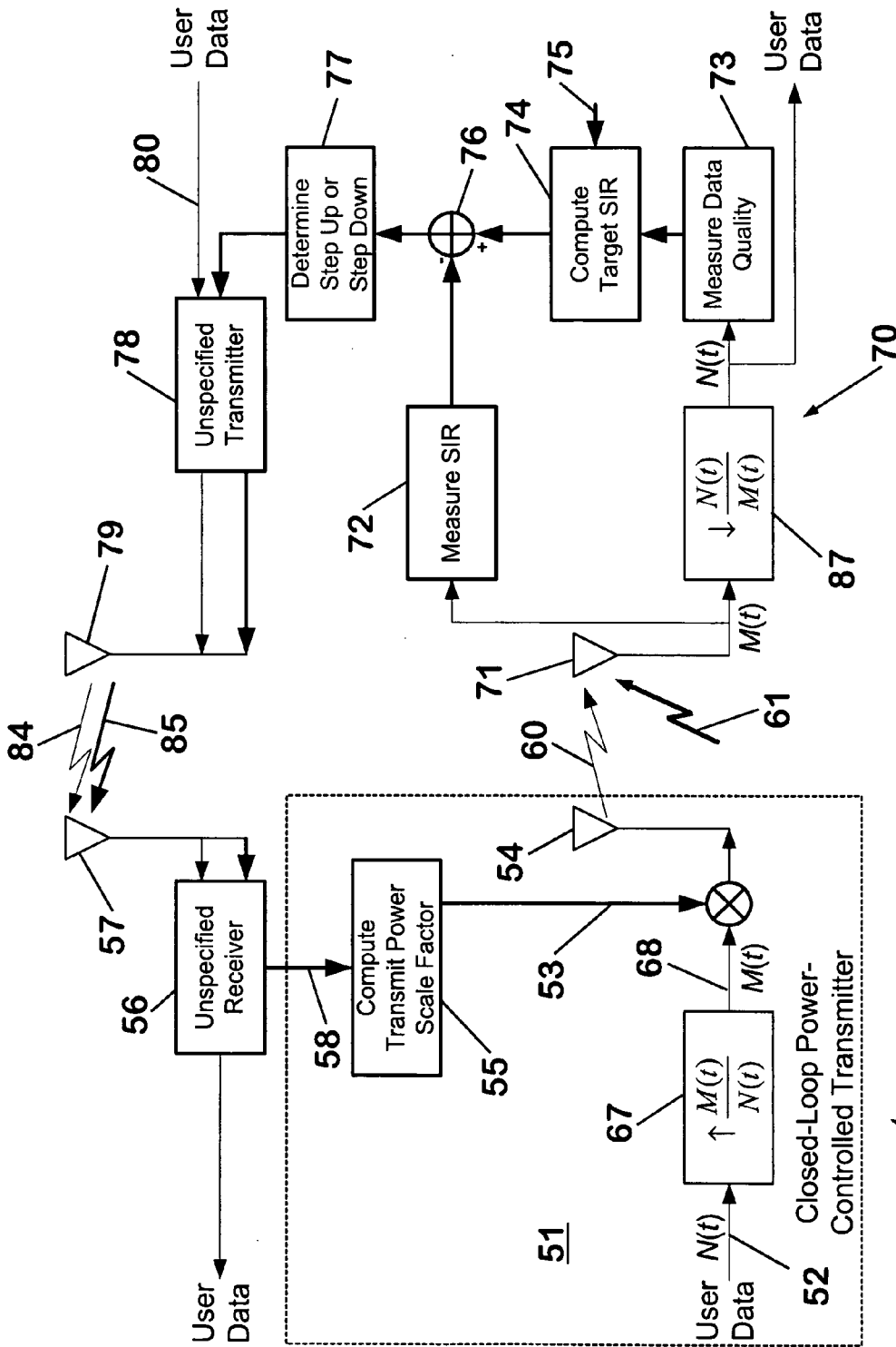
FIG. 4 (PRIOR ART)
