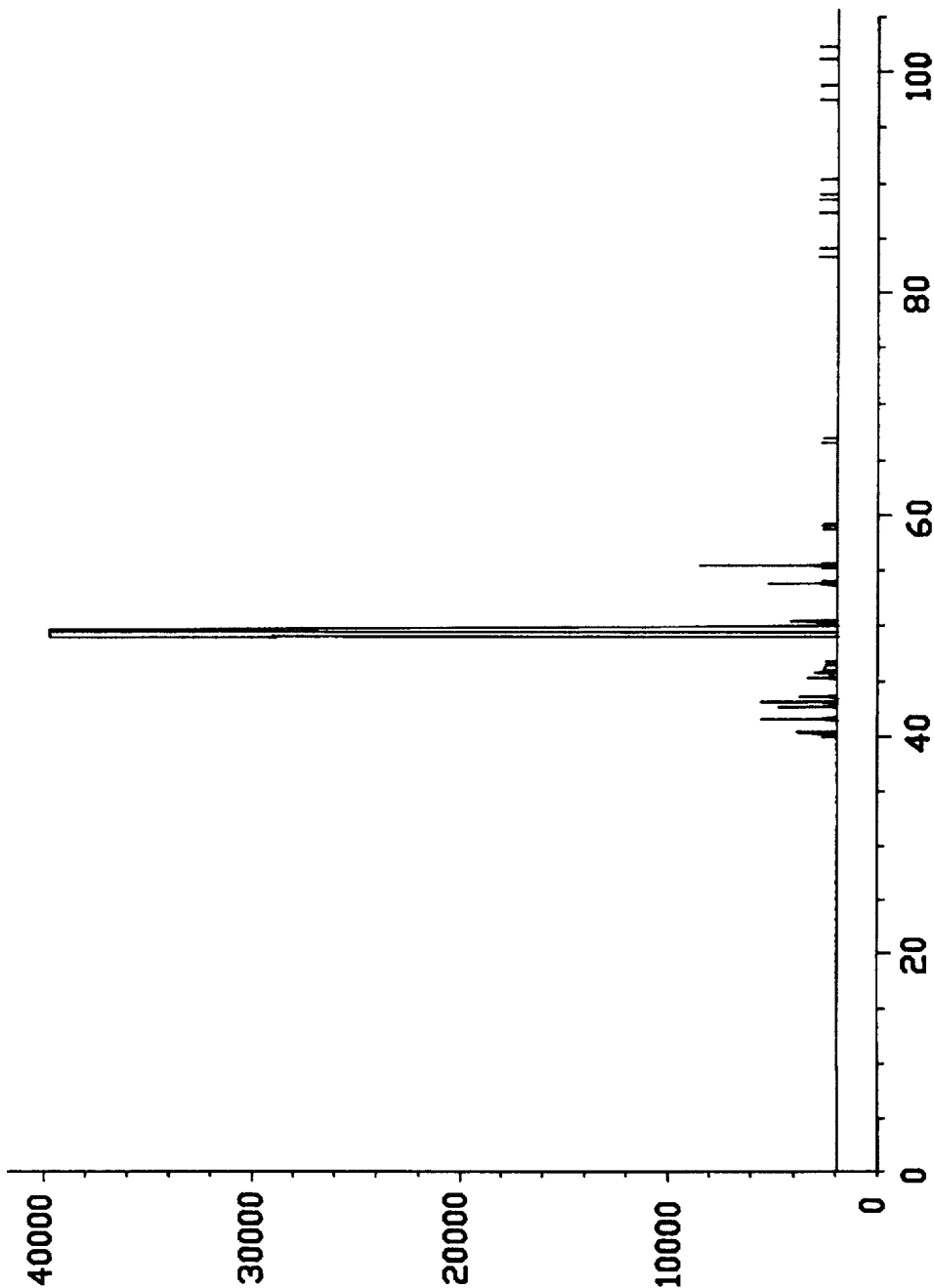
FIG. 4 GC PROFILE FOR EXAMPLE I(B)
