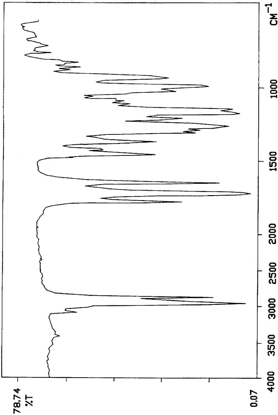
FIG.6 INFRARED SPECTRUM FOR EXAMPLE 1(B)
