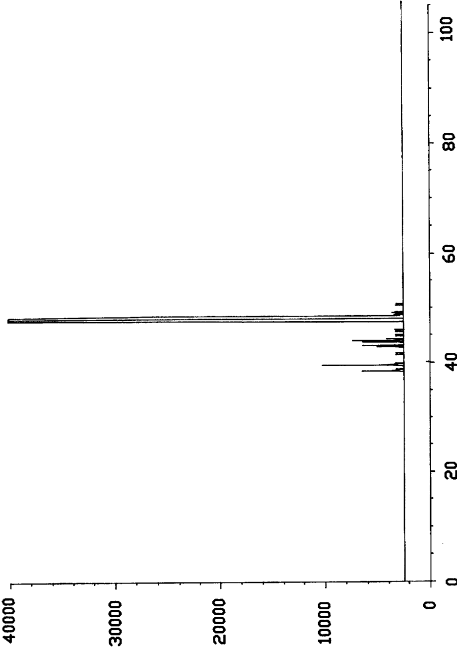
FIG.3 GC PROFILE FOR EXAMPLE 1(B)
