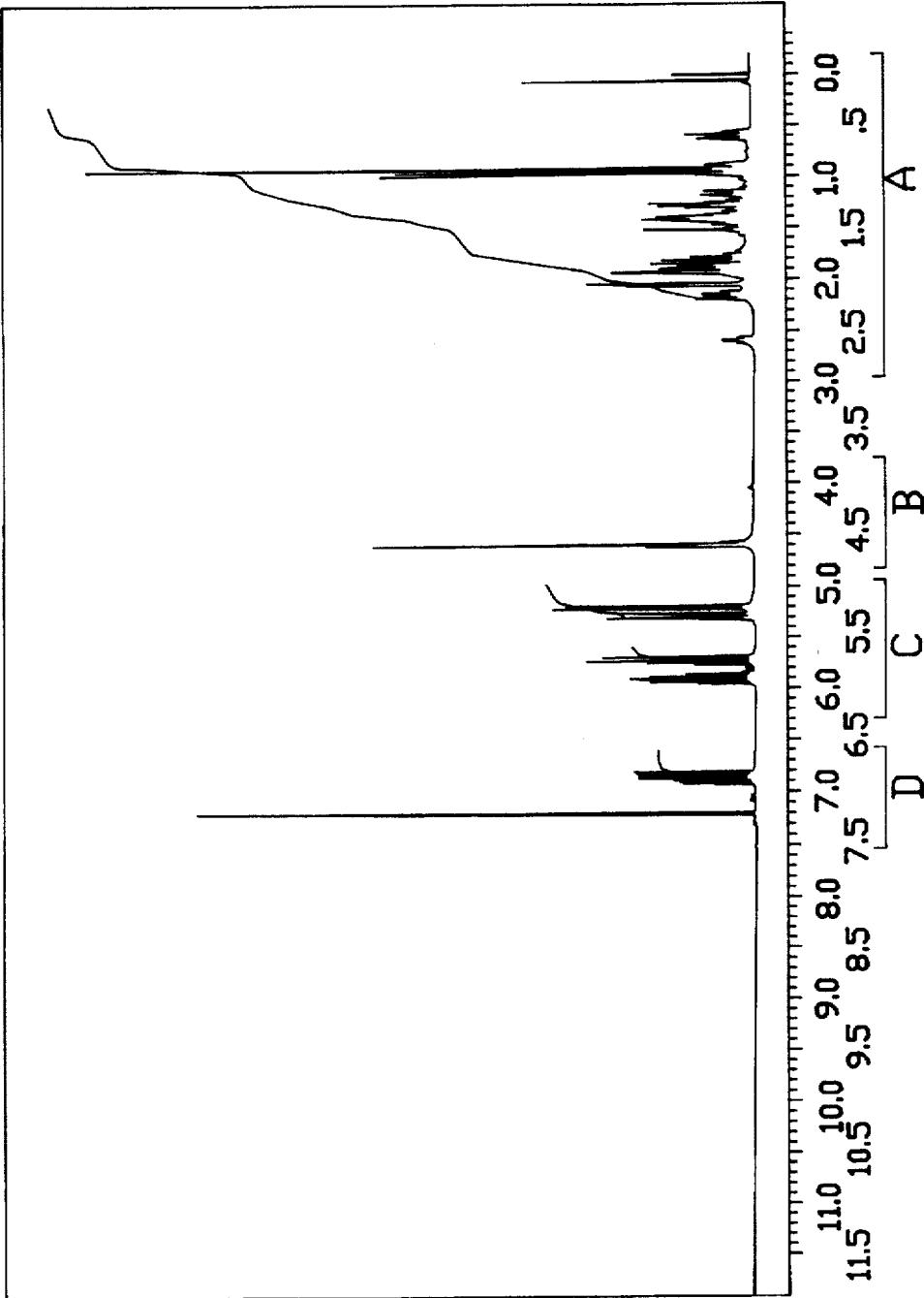
FIG.8 NMR SPECTRUM FOR EXAMPLE II
