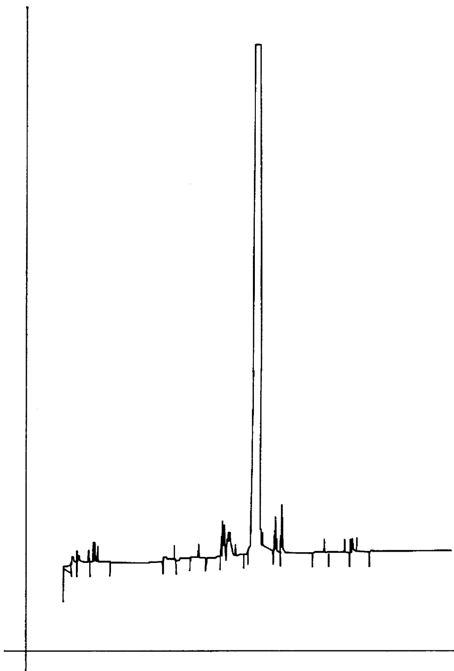
FIG.2 GC SPECTRUM FOR EXAMPLE I(B)
