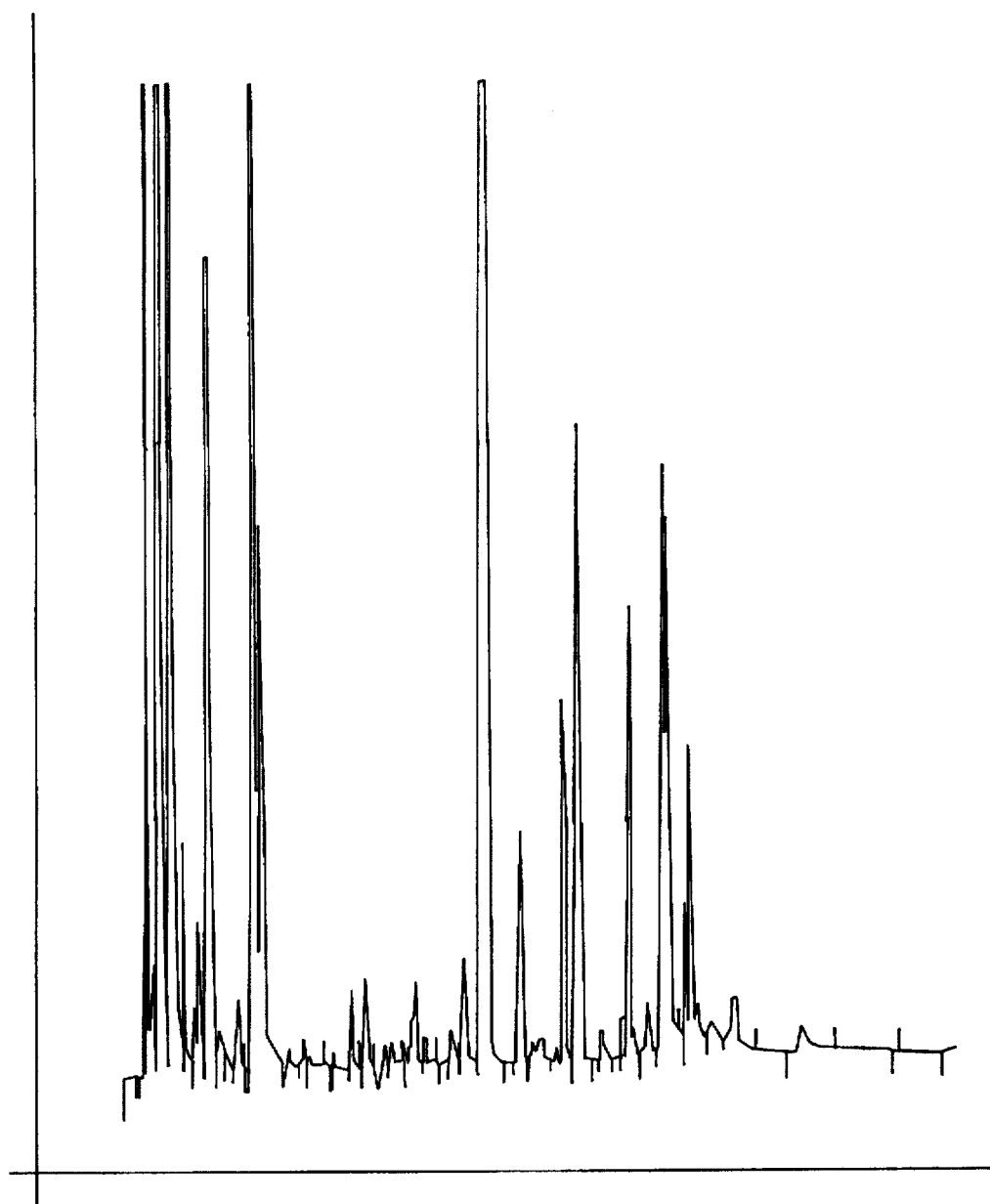
GC SPECTRUM FOR EXAMPLE III CRUDE
