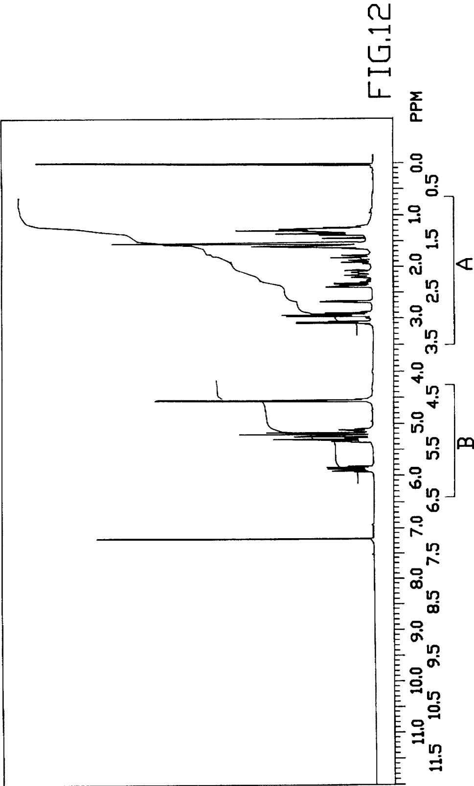
NMR SPECTRUM FOR EXAMPLE III
