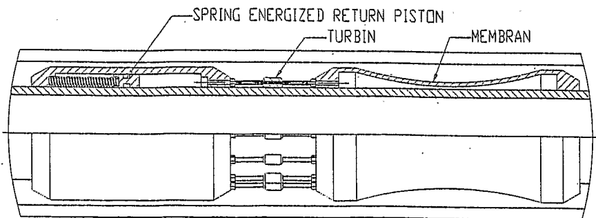
(J) PRESSURE ELECTRICAL GENERATION
