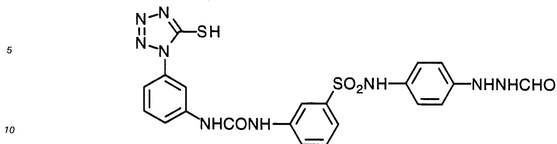
Hydrazine compound (1)
