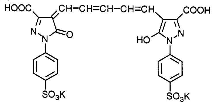
Compound C
