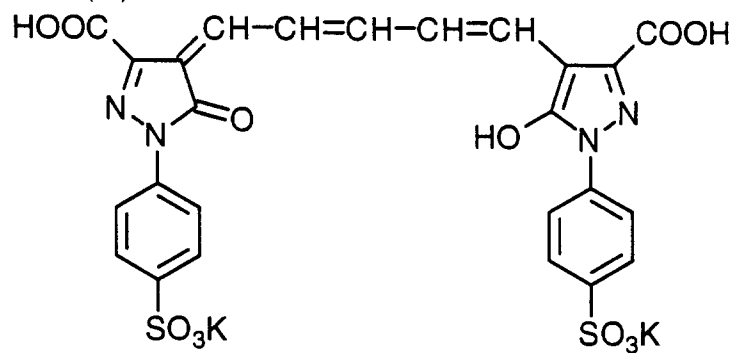
Compound (8)
