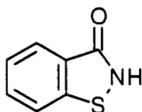
Compound A
