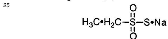
Compound (1)
