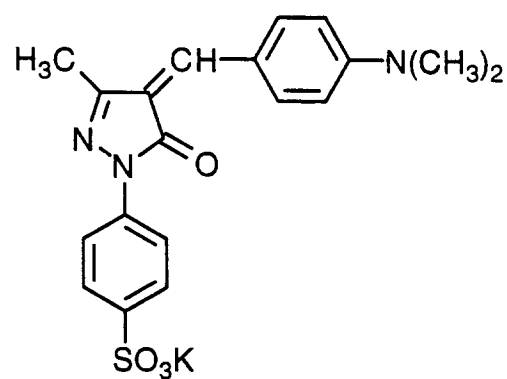
Compound (9)
