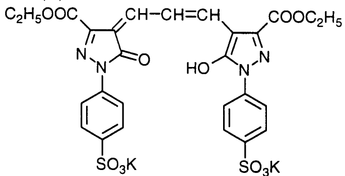
Compound (7)
