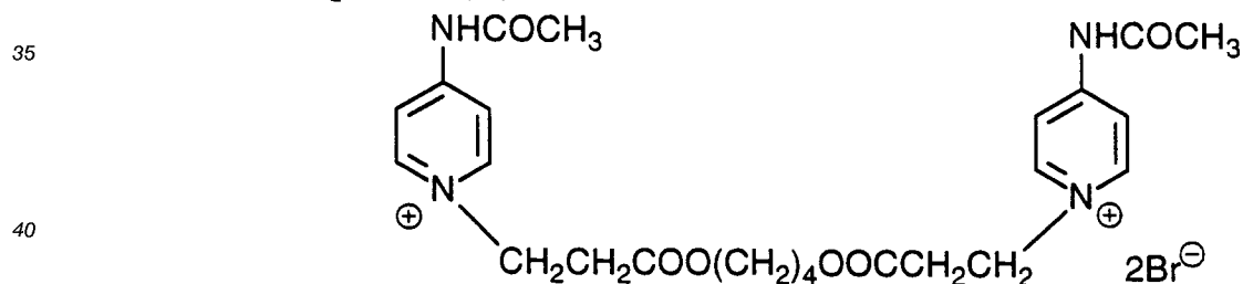
Compound (2)
