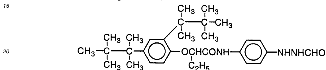
Hydrazine compound (2)
