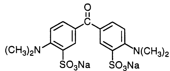
Compound (10)
