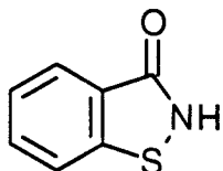
Compound (6)
