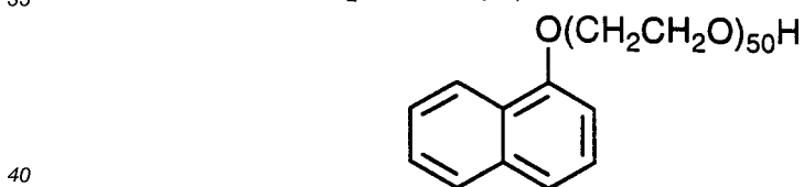
Compound (5)
