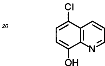
Compound (3)
