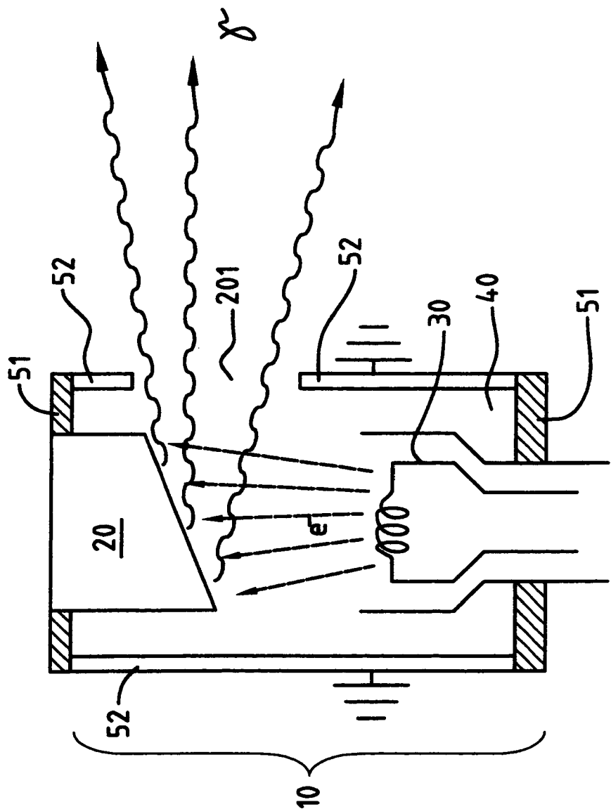
FIG. 3 (PRIOR ART)
