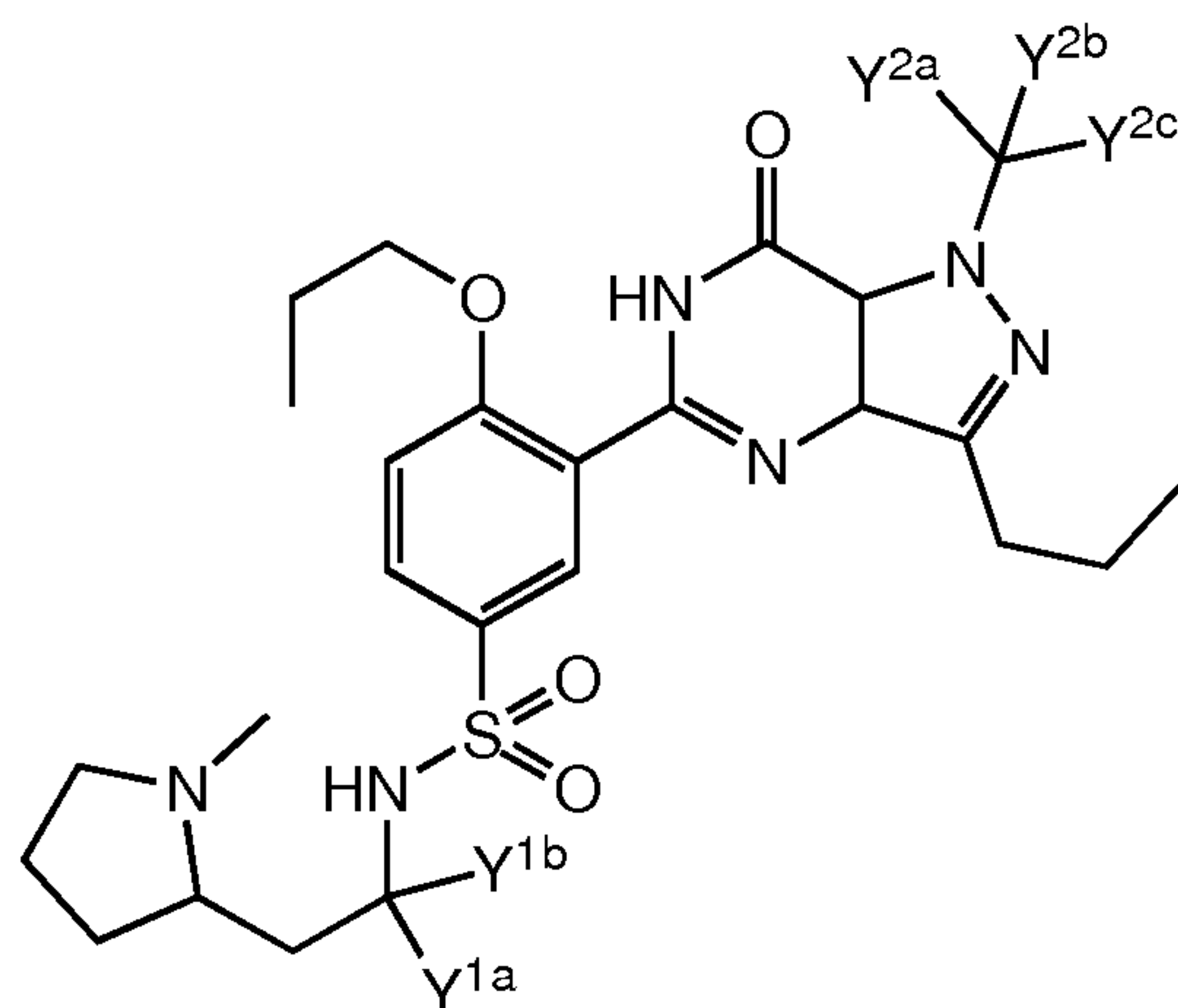
Formula (I)
