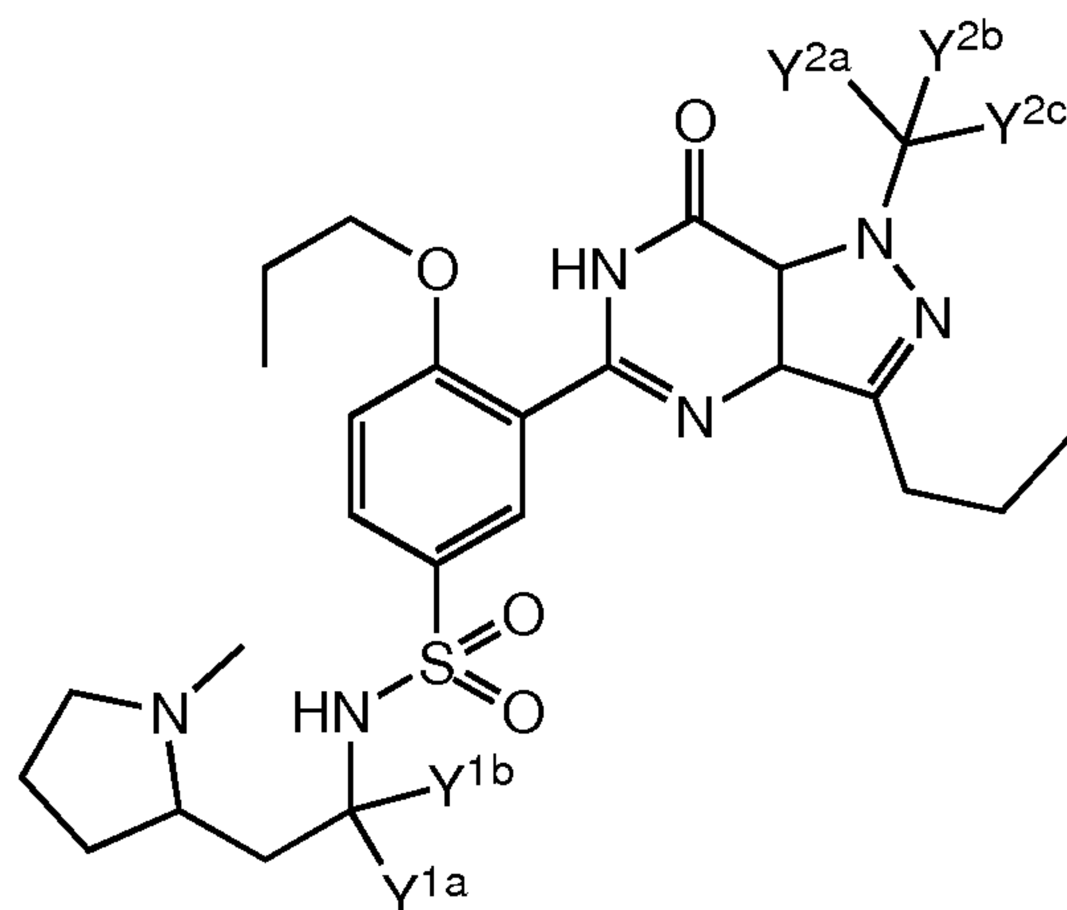
Formula (I)
