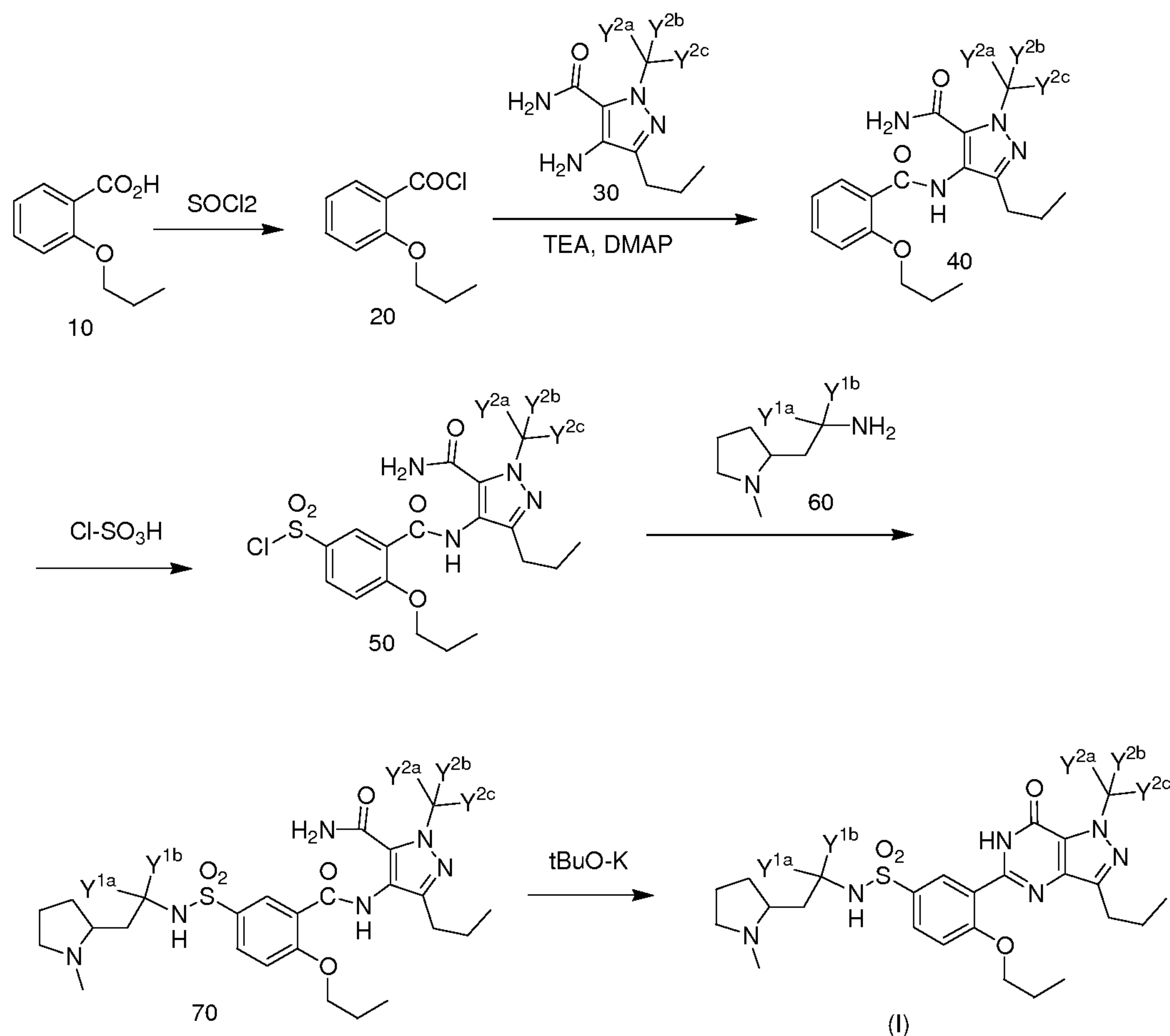
Scheme 1
