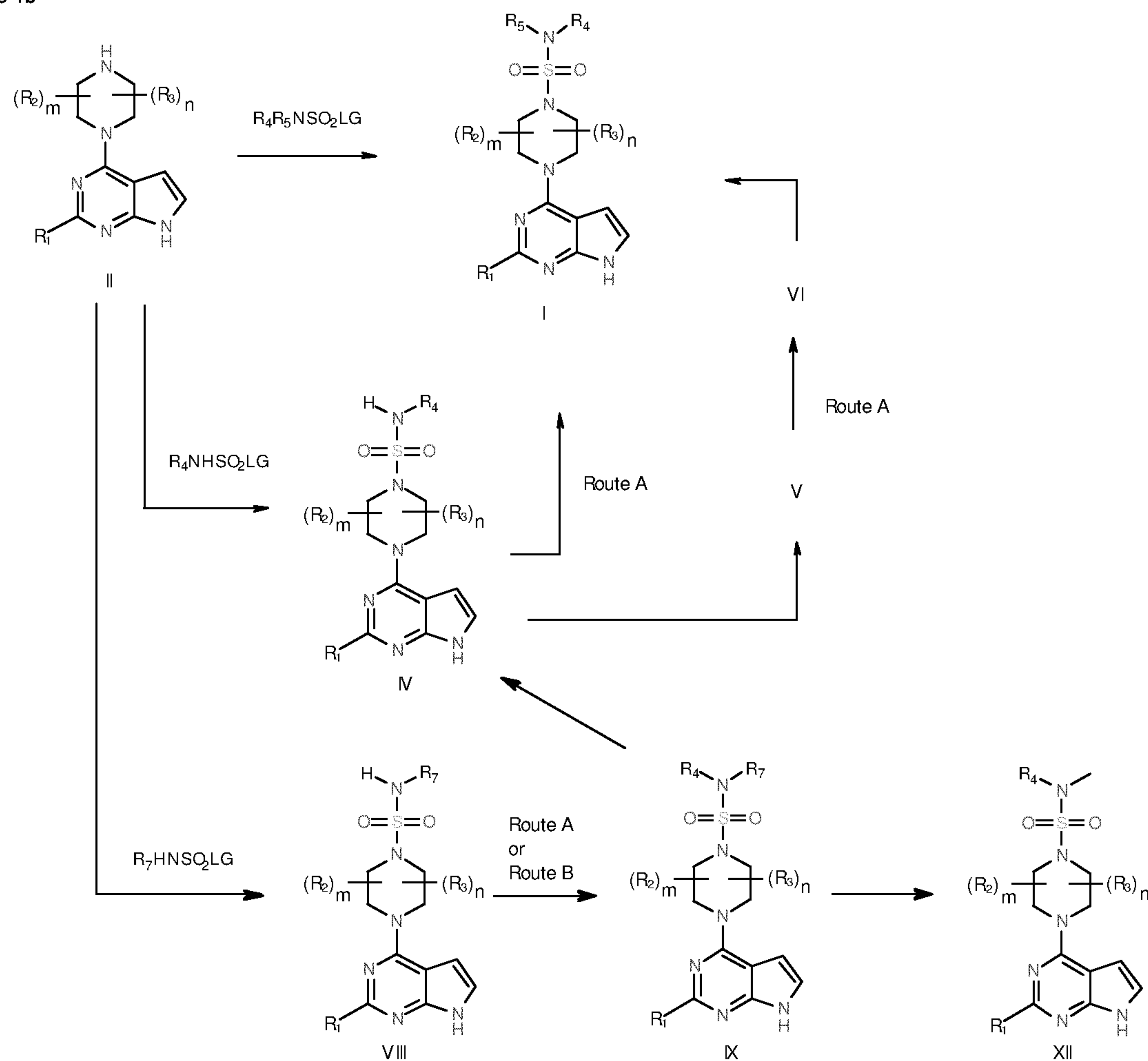
Scheme 1b
