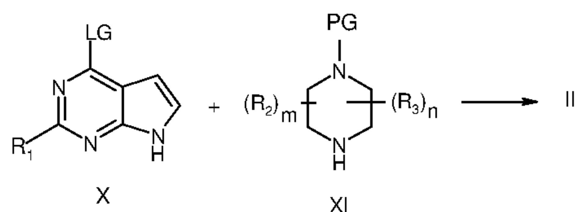
Scheme 2
