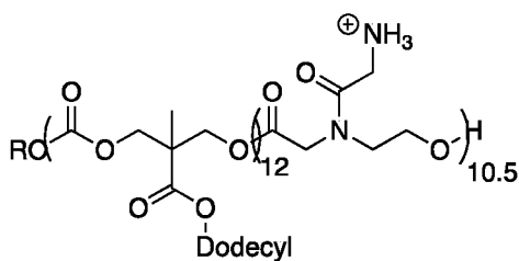
D 12 :Glycine 10.5
