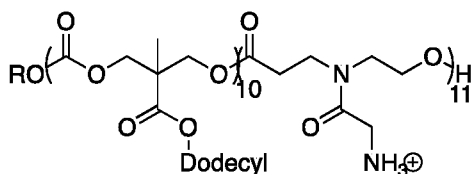
D 10 :(7-gly) 11
