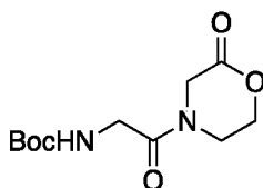
Glycine monomer
