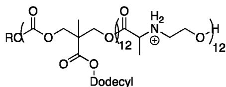
D 12 :Glu 12
