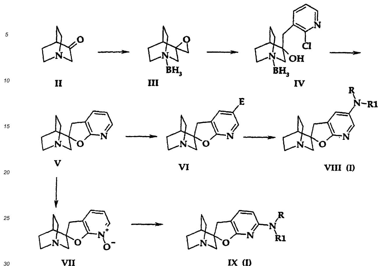
Scheme 1.
