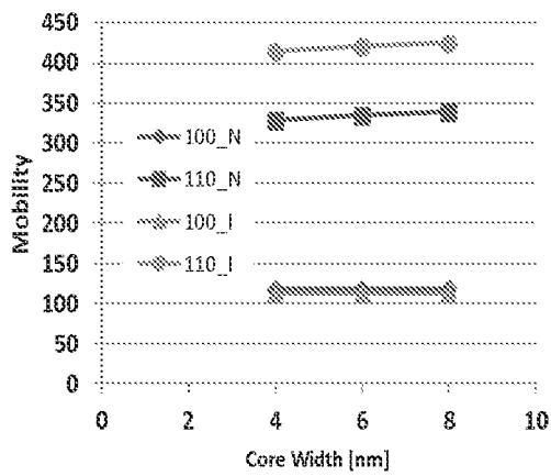
FIG. 21 Mobility
