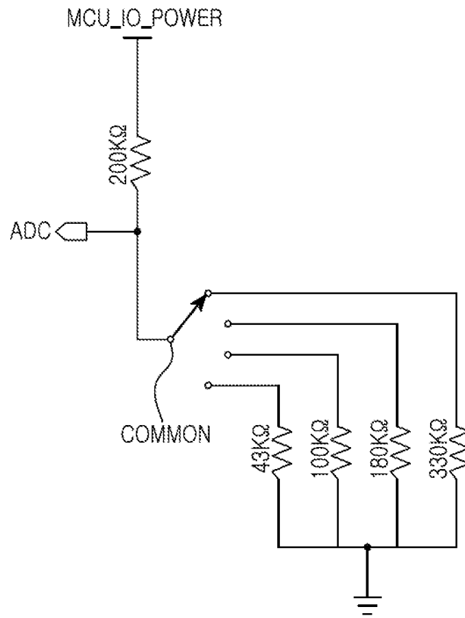
FIG.3 (CONVENTIONAL ART)
