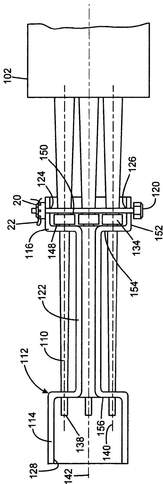
FIG. 6 PRIOR ART
