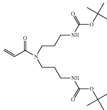
tert-butyl 3,3'-(acryloylazanediy)bis(propane-3,1-diyl)dicarbamate
