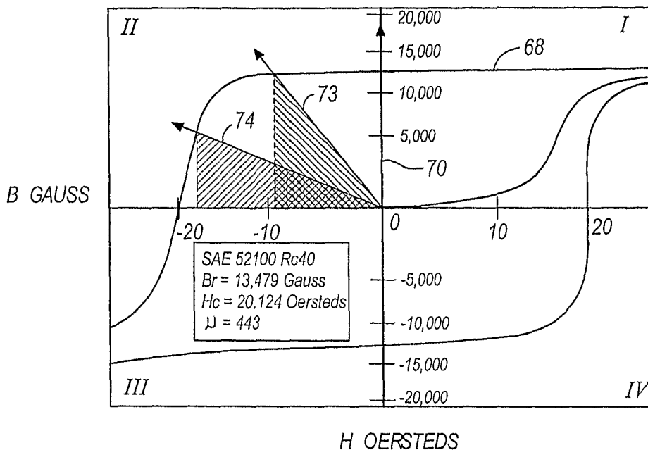
MAGNETIC HYSTERESIS CURVE SAE 52100 Rc40
