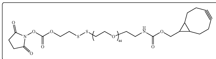
BCN—PEG-44-NHS
