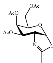
Compound 4
