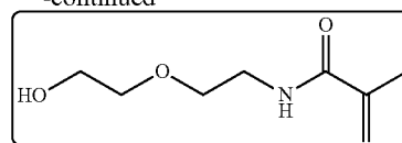
Compound 7
