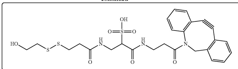
S—DBCO-disulfaneyl ethanol
