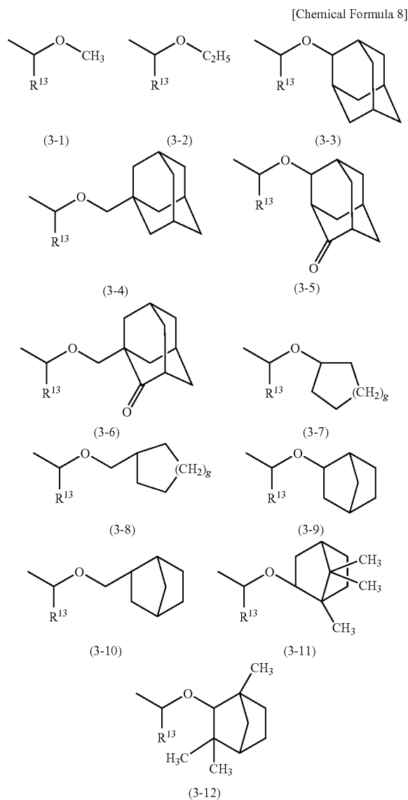
[Chemical Formula 7]
