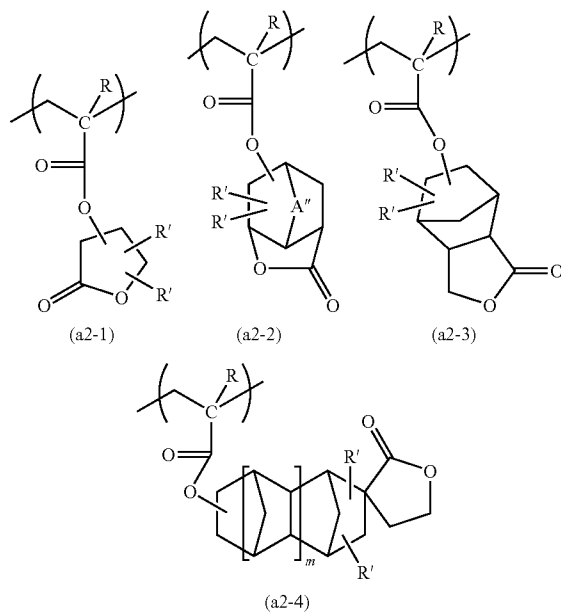
[Chemical Formula 23]
