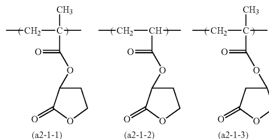
[Chemical Formula 24]
