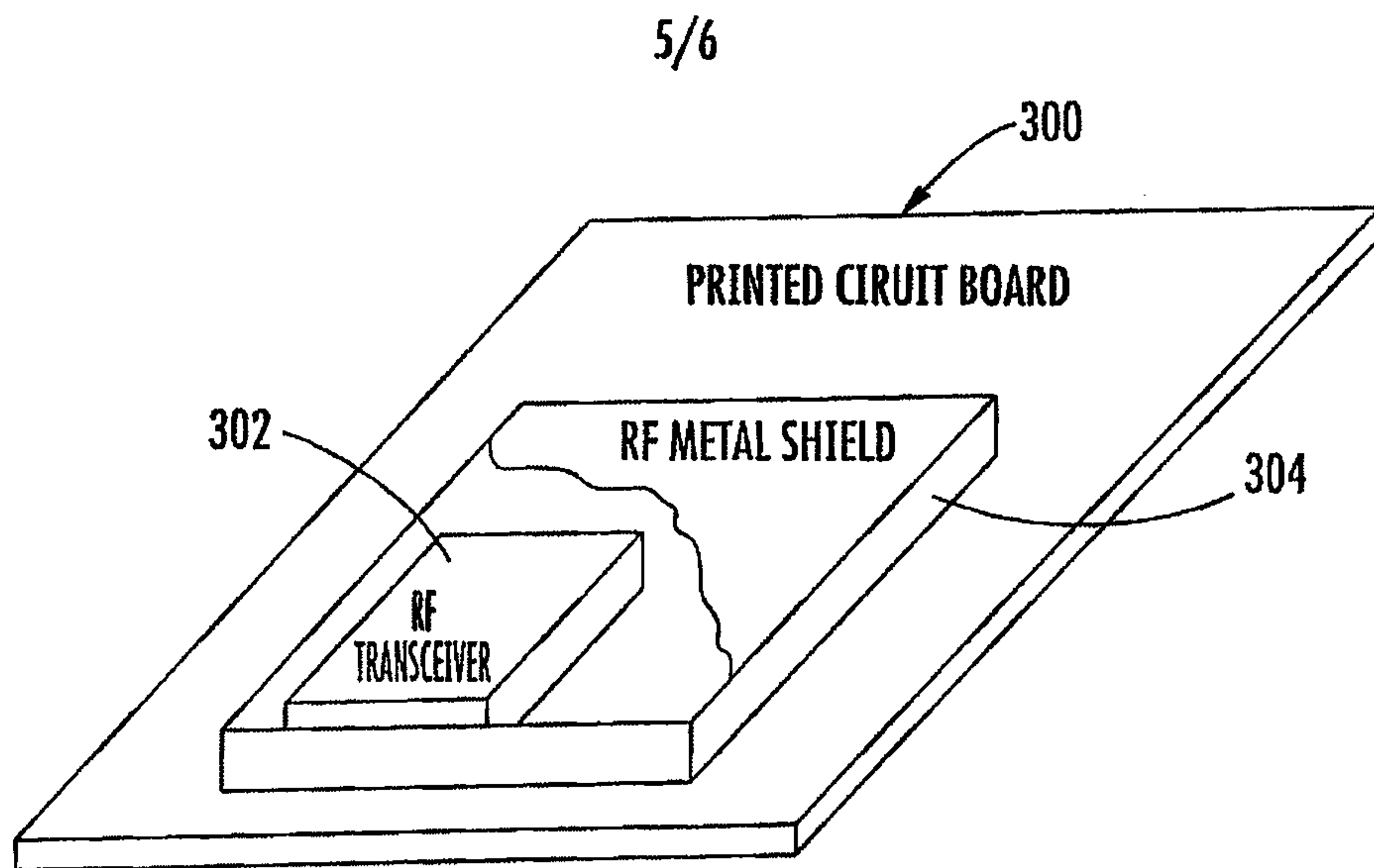
FIG. 5 (PRIOR ART)
