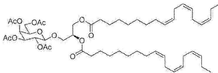
Chemical Formula: C_{53}H_{82}O_{14} Molecular Weight: 943.23.
