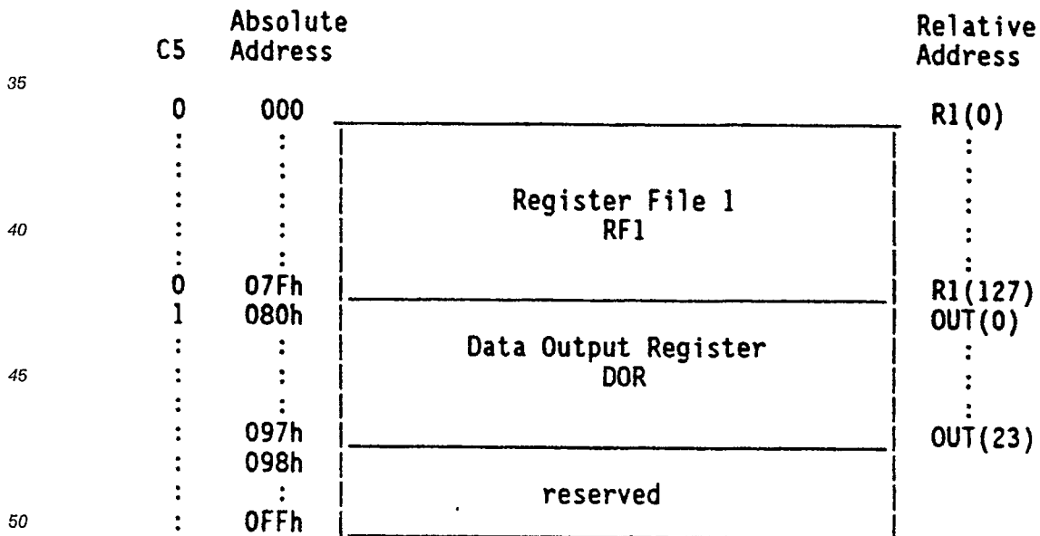
DOR/RF1 Memory Map: h indicates hexadecimal
